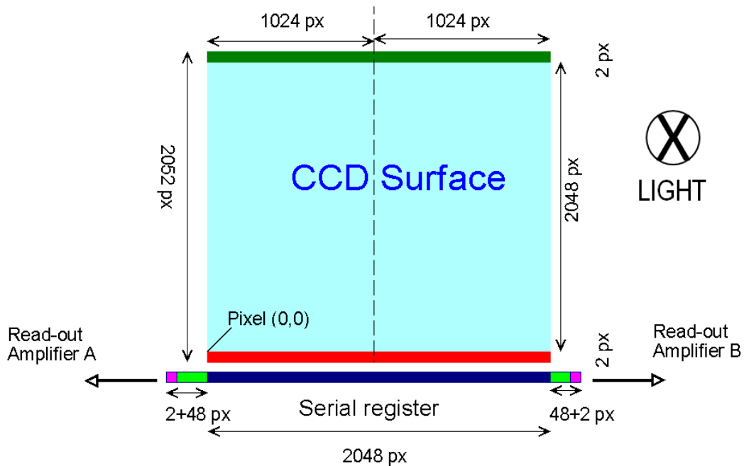
Figure 5: CCD array as seen by the science beam. CCD and S/C coordinate systems are shown
