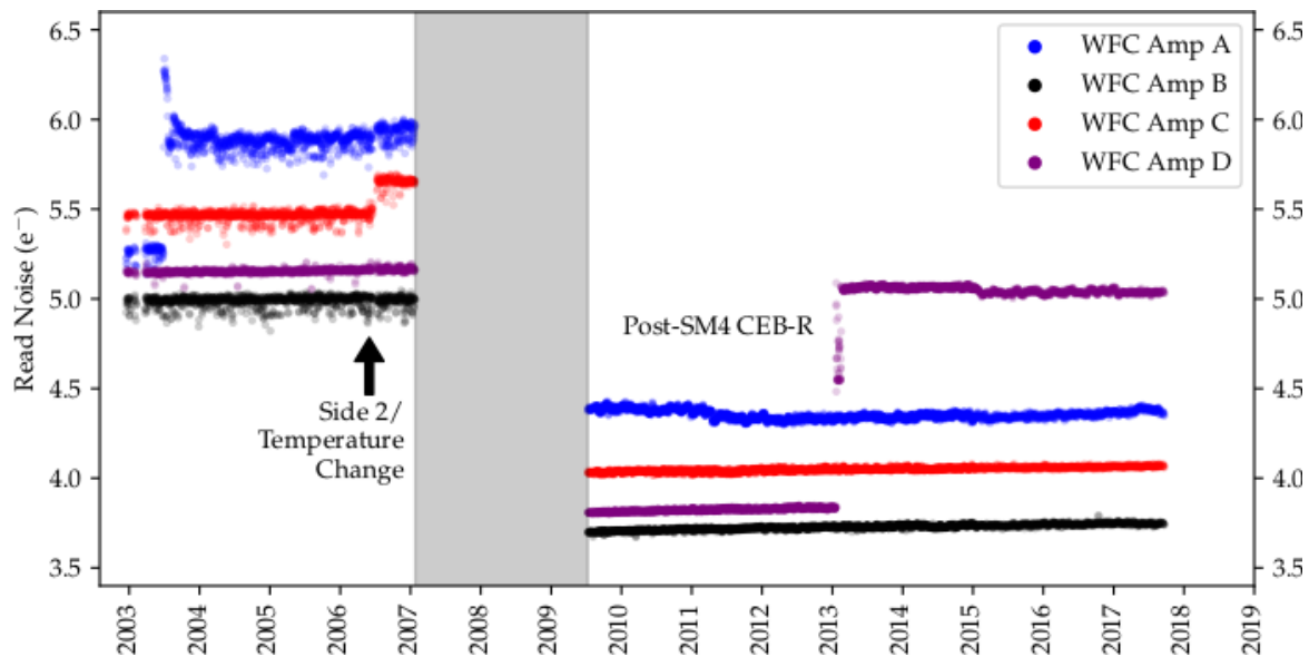
Figure 4.1: History of the amplifier-based read noise (in electrons).
