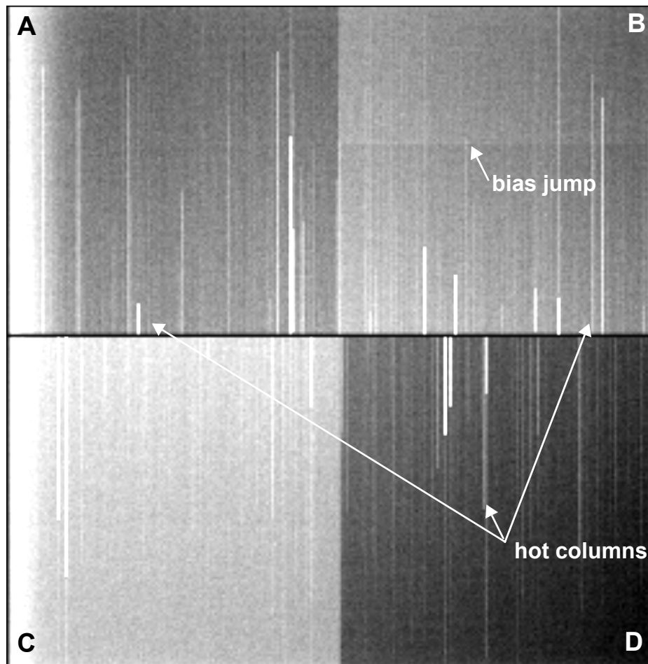
Figure 4.6: Bias Jump in the WFC1 Quadrant B Only
