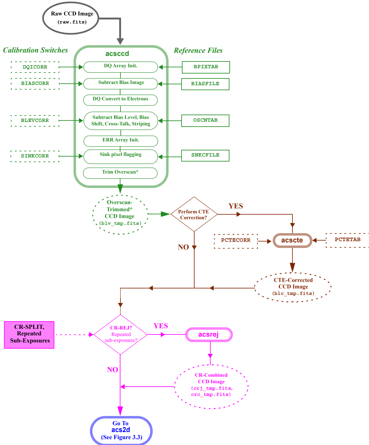
Figure 3.2: Flow Diagram for CCD Data Using acsccd and acscte in calacs
