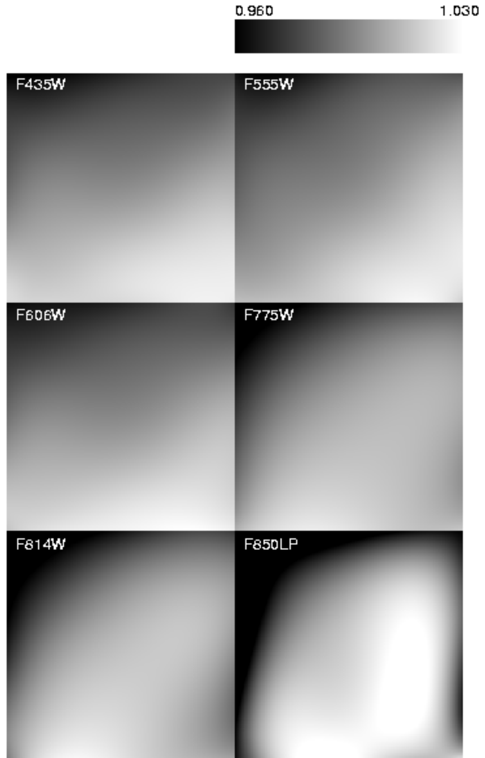
Figure 4.19: SBC Low Frequency (L-flat) Flat-Field Corrections Required for the In-flight Deuterium Lamp Data
