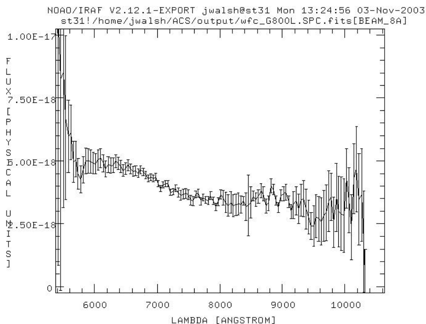
Figure 5.11: Example WFC G800L Extracted Spectrum
