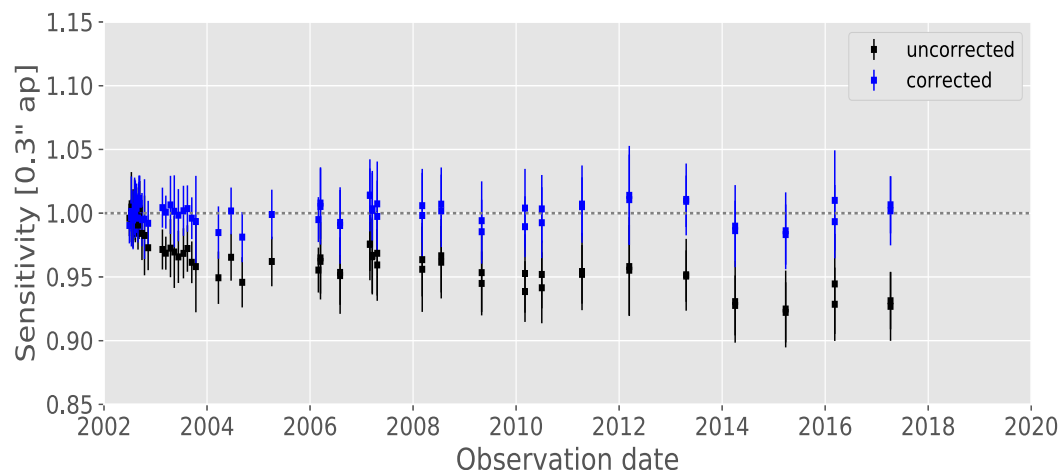
Figure 5.4: Sensitivity of the F125LP imaging mode, as a function of time. Error bars represent 1 sigma scatter in the sensitivity relative to the reference photometry.
