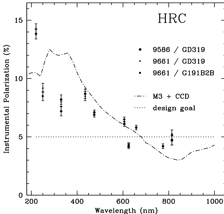
Figure 5.5: Instrumental Polarization for the HRC
