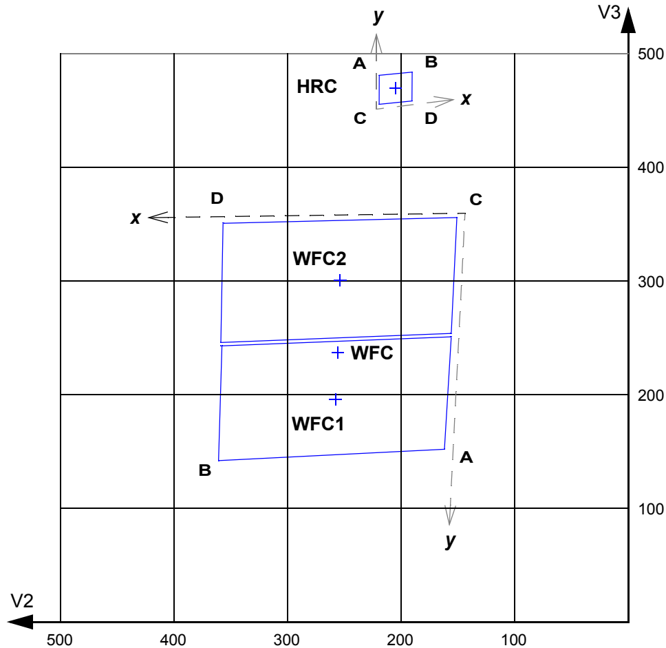
Figure 1.1: WFC and HRC Apertures Compared with the V2/V3 Reference Frame
