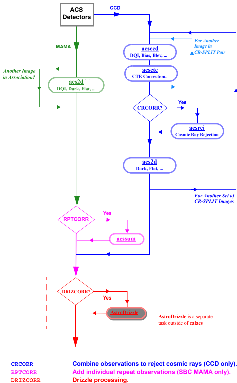
Figure 3.1: Flow Diagram for ACS Data, With calacs Task Names
