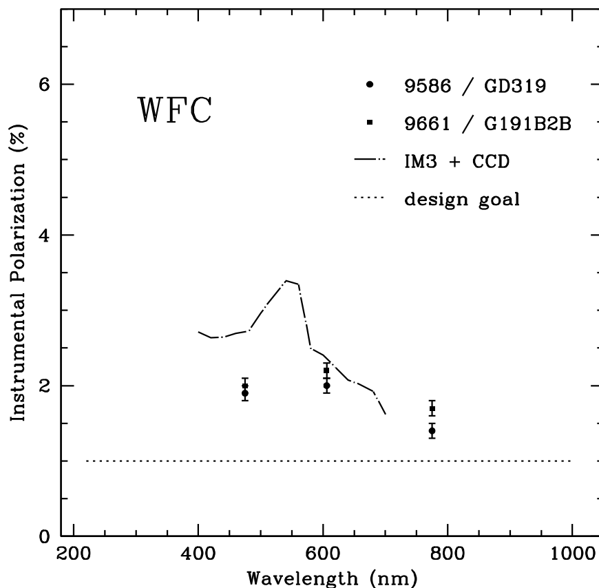
Figure 5.6: Instrumental Polarization for the WFC
