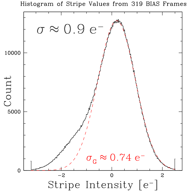
Figure 4.5: Characterization of the Low-level 1/f Noise from WFC Bias Frames
