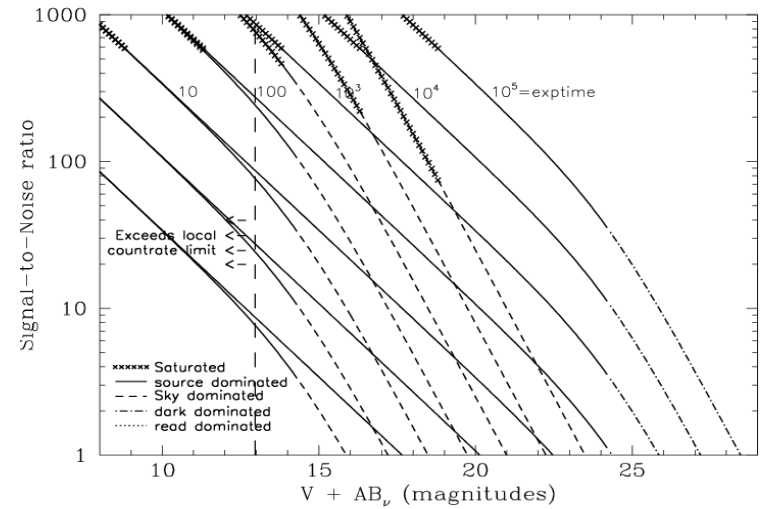
Figure 10.108: Extended source S/N vs. V+AB_v for the SBC/F122M filter. Top curves are for low sky and bottom curves are for average sky for a 1 \text{ arcsec}^2 area.
