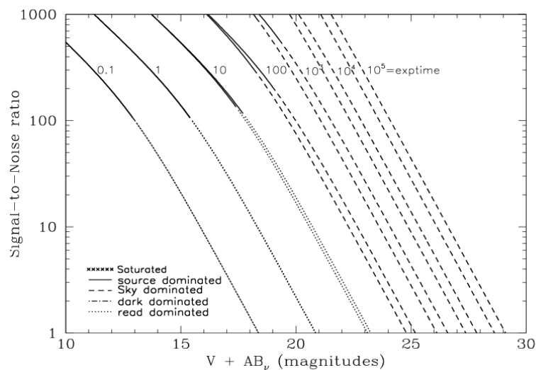
Figure 10.18: Extended source S/N vs. V+AB_v for the WFC/F606W. Top curves are for low sky and bottom curves are for average sky for a 1 arcsec 2 area.
