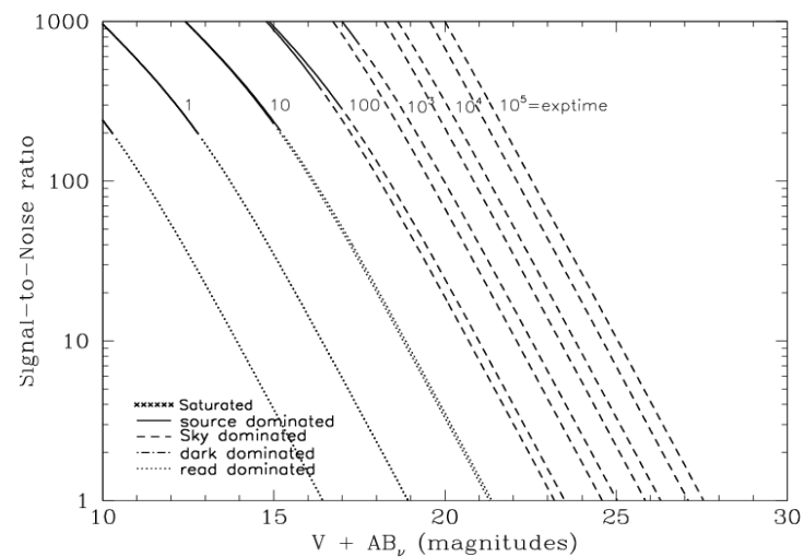
Figure 10.87: Extended source S/N vs. V+AB_v for the HRC/F814W filter. Top curves are for low sky and bottom curves are for average sky for a 1 arcsec 2 area.
