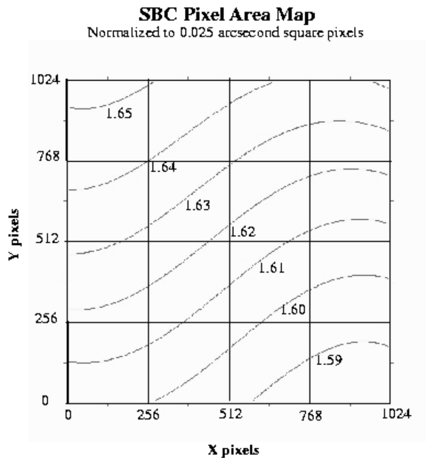
Figure 10.132: The map of the effective pixel areas of the ACS/SBC. The areas are normalized to 0.025 arcsecond square pixels.
