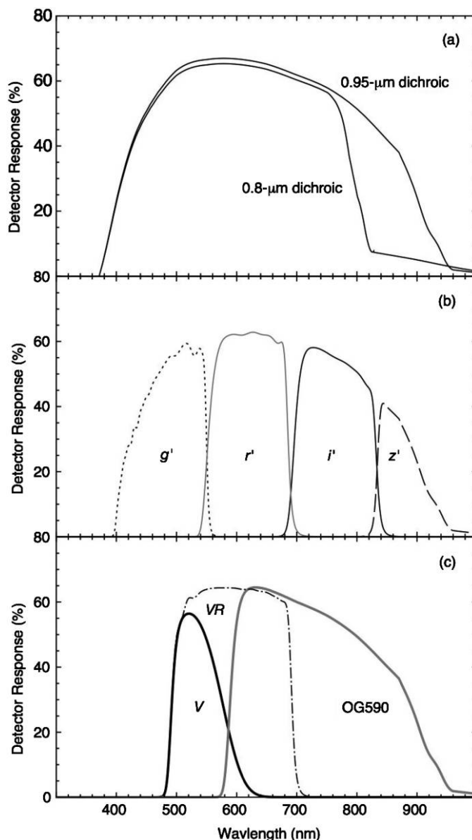
FIG. 4.—The MORIS detector response as a function of wavelength. The response is shown as a percentage of light entering the telescope and thus includes throughput from all optics, as well as CCD quantum efficiency. (a) Response with no filter. The two curves correspond to the SpeX 0.8\ \mu\text{m} and 0.95\ \mu\text{m} dichroic beam splitters, one of which must be selected to direct light out of the side-facing exit window and into the MORIS fore optics box. (b) Response for the Sloan filters, with the 0.95\ \mu\text{m} dichroic. Sloan g' , r' , i' , and z' are represented by dotted, gray, black, and dashed lines, respectively. (c) Response for the remaining filters, with the 0.95\ \mu\text{m} dichroic. Johnson V , VR , and long-pass red (OG590) are represented by thick black, dot-dashed, and thick gray lines, respectively.
