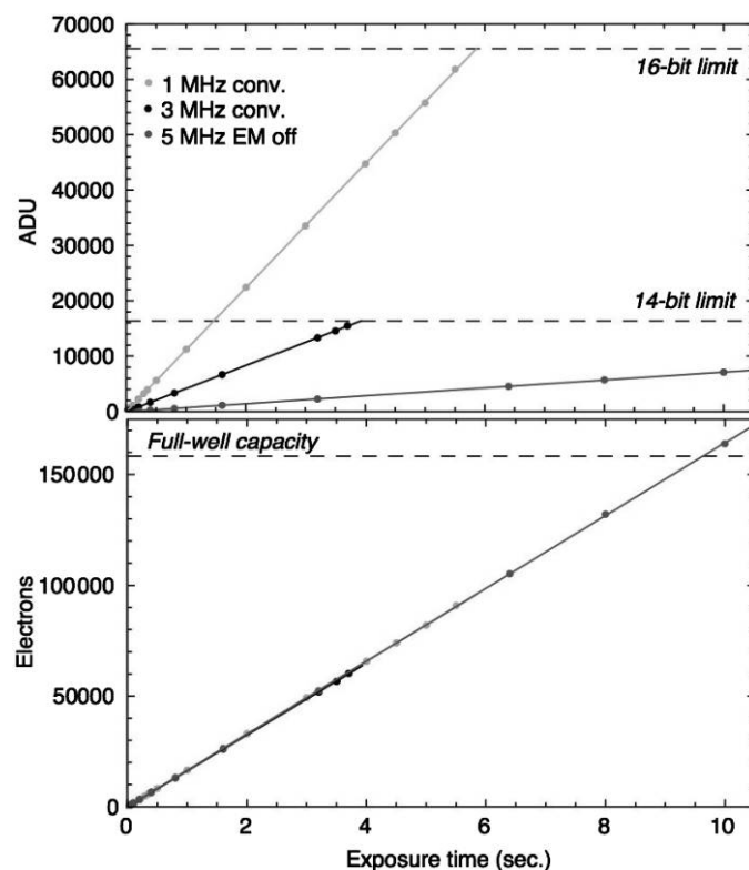
FIG. 2.—MORIS linearity measurements of an evenly illuminated field. The average bias-subtracted counts per pixel are plotted vs. time, along with best-fit lines. Three modes were tested: 1 MHz conventional 2.4× (16-bit; 1.47 e^- \text{ ADU}^{-1} ), 3 MHz conventional 2.4× (14-bit; 3.89 e^- \text{ ADU}^{-1} ), and 5 MHz EM off 2.4× (14-bit; 23.05 e^- \text{ ADU}^{-1} ). Horizontal dashed lines represent saturation limits. The conventional modes reach saturation due to the data transfer limitation of the ADC, while the EM mode reaches saturation slightly past the manufacturer's specified full-well capacity. All data lie within 1% of the best-fit lines.
