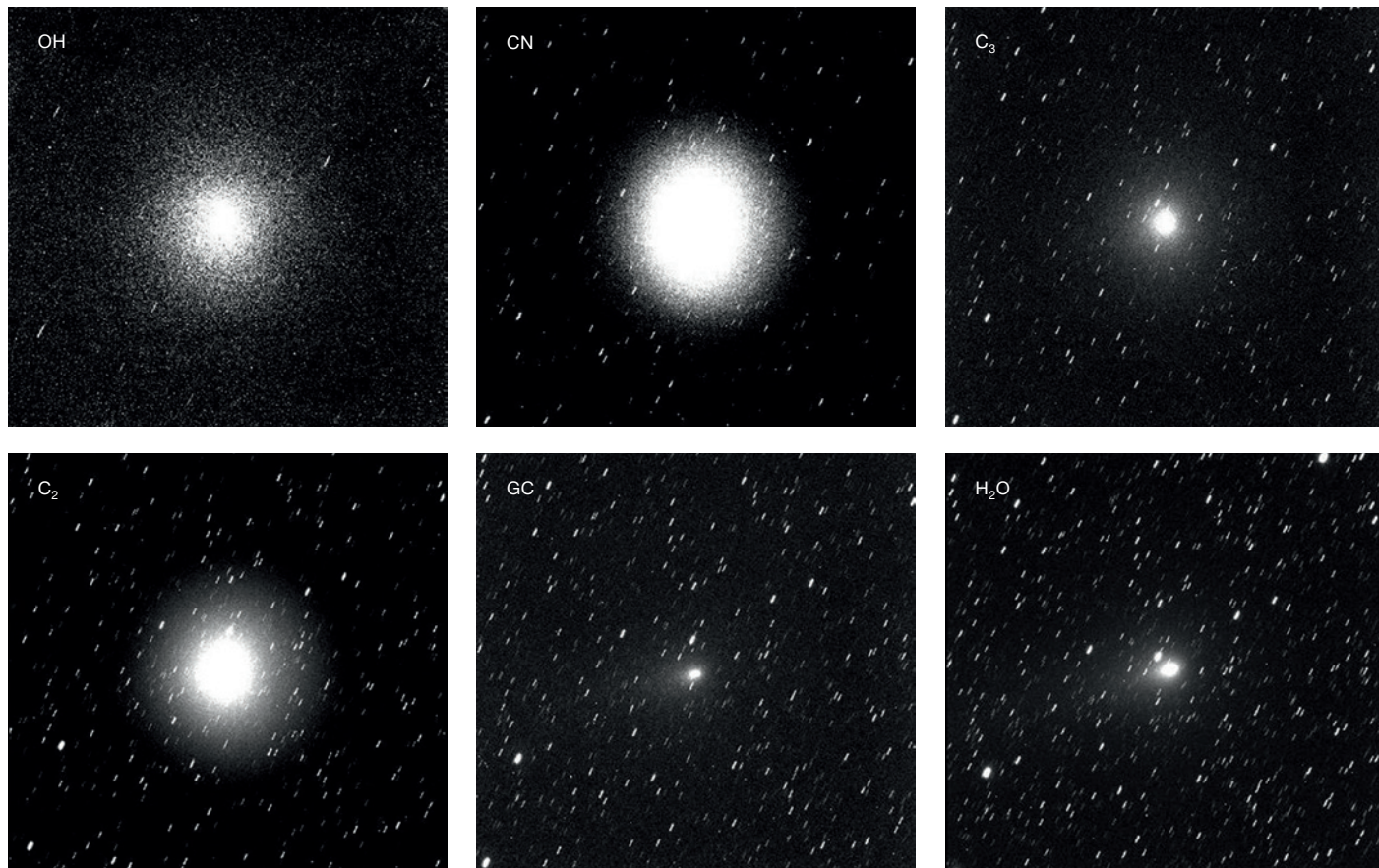
Figure 4. Comet 103P/Hartley 2 imaged with TRAPPIST through the different cometary filters on 5 November 2010: OH, CN, C 3 , C 2 , green continuum (GC) and H 2 O + . Note the different shapes and intensities of the cometary coma in each filter.
