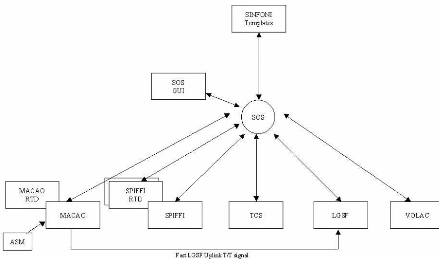
Figure 23: SINFONI software overview
