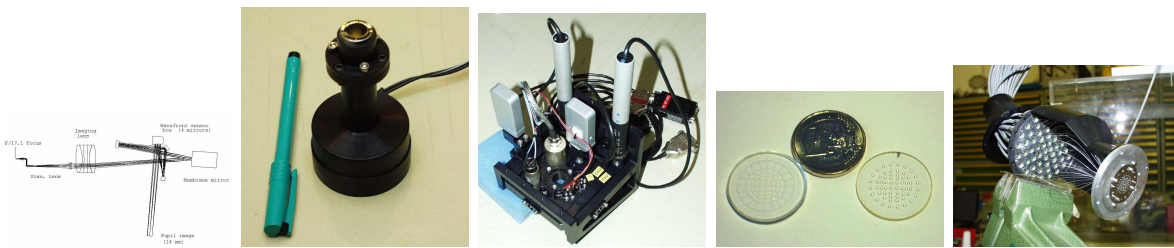
Figure 14: WFS optics – Membrane mirror – Gimbal mount – Lenslet array – Fiber module
