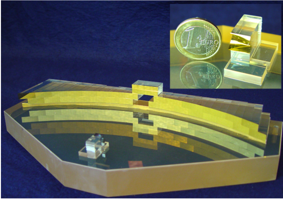
Figure 20: SPIFFI image slicer (a): The light enters through the hole in the big slicer. A stack of 32 small mirrors, the small slicer (also shown in the sub-panel), slices the image and redirects the light towards the 32 mirrors of the big slicer, which re-arranges the slitlets into a 31 cm long pseudo-slit.
