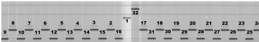
Figure 21: The layout of the slitlets on a raw SPIFFI frame.
