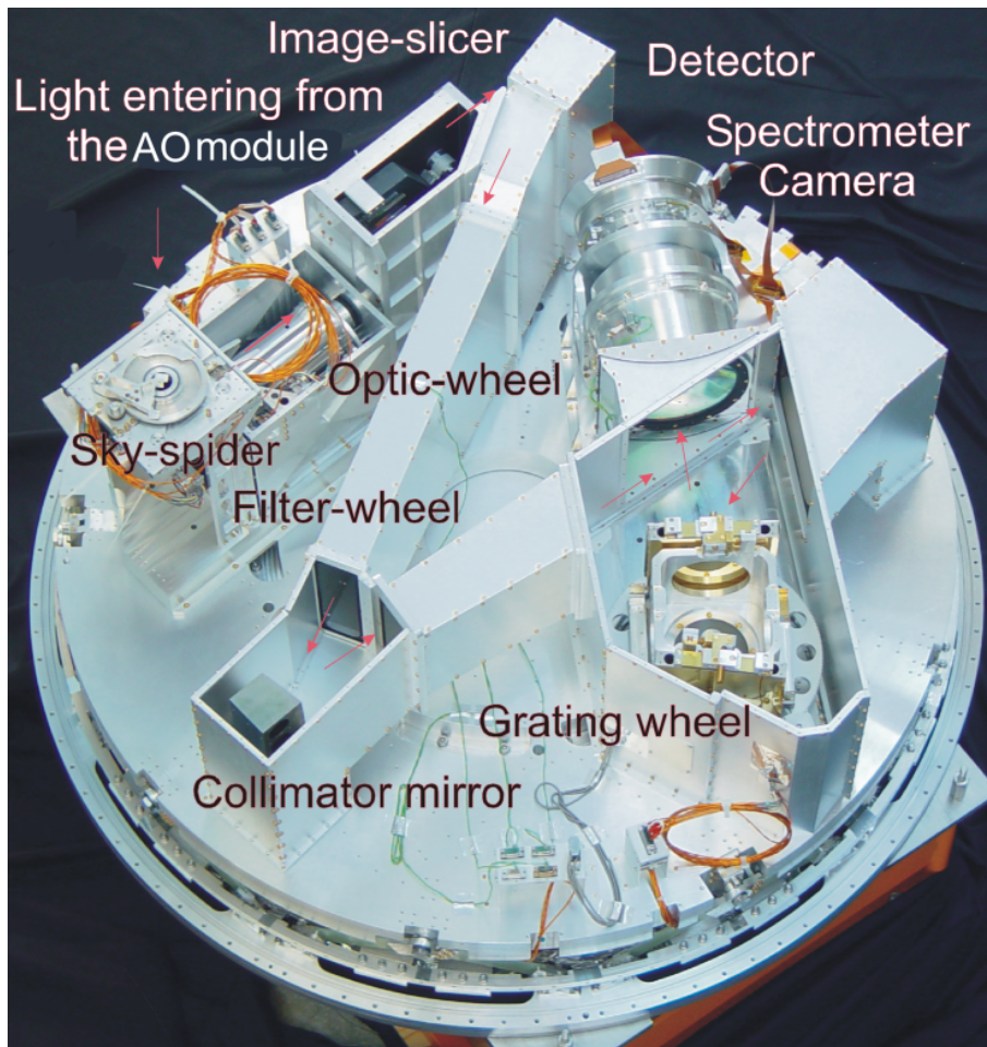
Figure 19: An inside view of SPIFFI: The cryostat cover and the reinforcing structure have been removed to provide a free view on the opto-mechanical components of SPIFFI. The light enters from the top, and passes the sky-spider. The pre-optics with a filter-wheel and interchangeable lenses provides three different image scales. The image slicer re-arranges the two-dimensional field into a pseudo-long slit, which is perpendicular to the base plate. Three diamond turned mirrors collimate the light onto the gratings. In total, four gratings are implemented on the grating drive. A multiple-lens system then focuses the spectra on a Rockwell HAWAII array. The diameter of the instrument is 1.3m.
