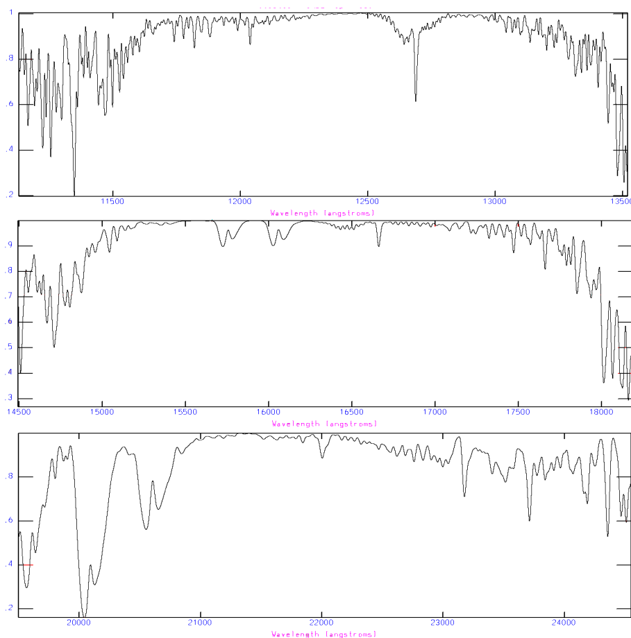
Figure 9: Atmospheric transmission in the J, H and K bands. These graphs are based on FTS data from Kitt Peak, produced by NSF/NOAO.
