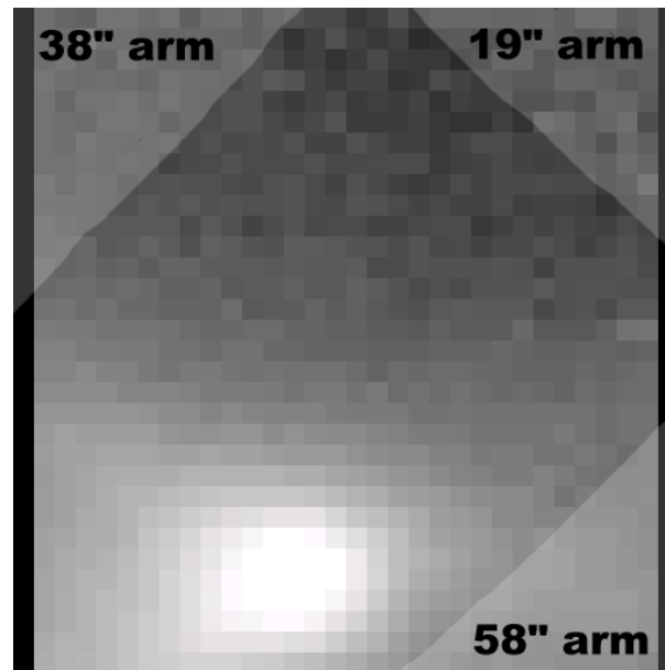
Figure 22: The positions of the sky-spider arms on the SPIFFI FOV. NB: only one arm may be used at a time and its coverage of the field is user selectable.
