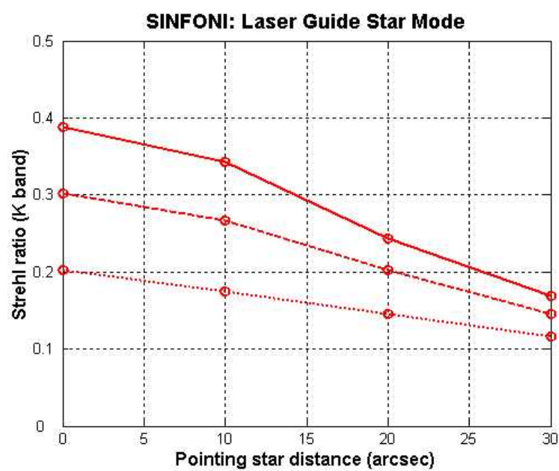
Figure 18: LGS Strehl performance
