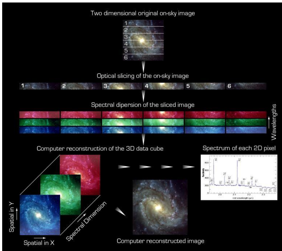
Figure 10: The function of the image slicer. The field of view (top) is sliced into small slices which are recombined into a pseudo longslit before being dispersed. The dispersed planes can be recombined to form an image, or used to extract a spectrum at any position within the field of view. Note that for SINFONI, slice number 1 corresponds to the BOTTOM slice in the FOV, and the slice number increases upwards (i.e. the opposite to the graph above). Also, on the detector the wavelength increases downwards (not upwards as in the graph above).
