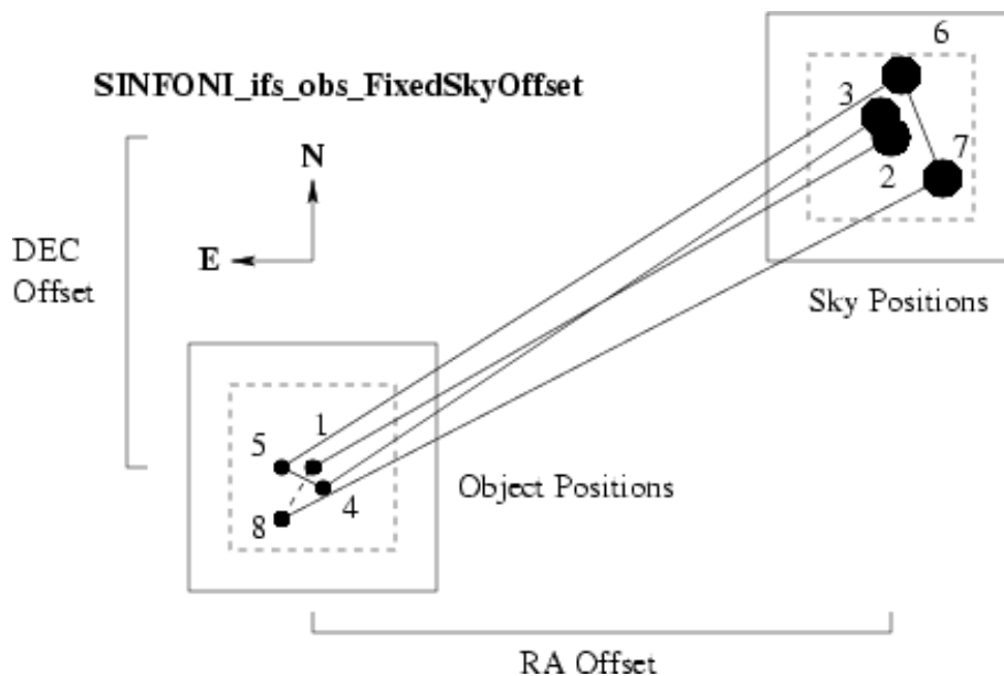
Figure 25: An illustration of the offset sequence taken with the FixedSkyOffset template. (“Number of exposure per Offset” = 1). The large circles for the sky position indicate that these observations are performed in open loop.
