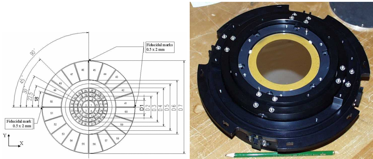
Figure 13: DM electrode geometry – DM/TTM assembly
