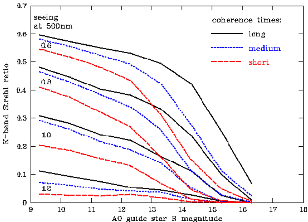
Figure 17: NGS performance for a wide range of optical seeing values (0.6 to 1.2'' ) and long, medium and short coherence times.
