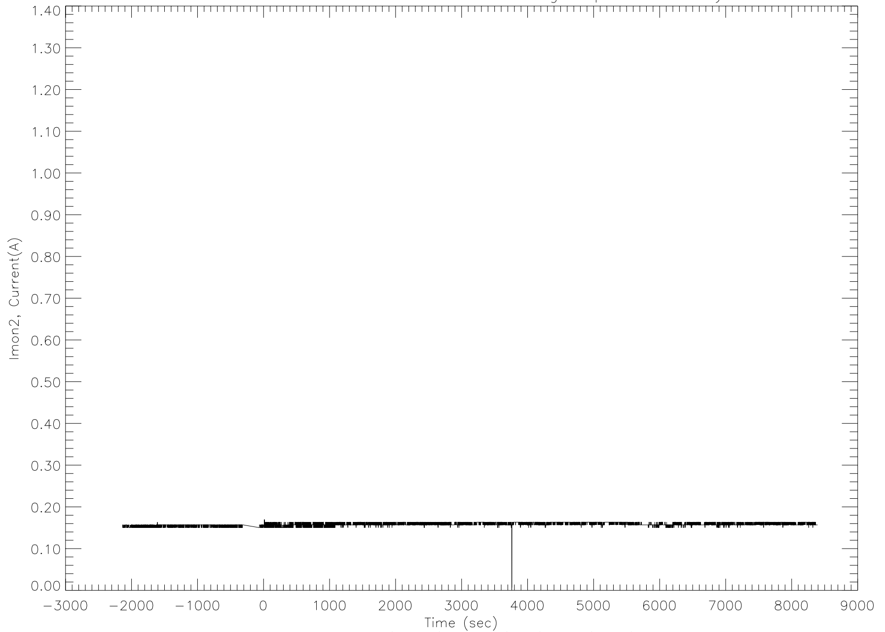
GCMS Protected Current vs MET from High-Speed Telemetry
