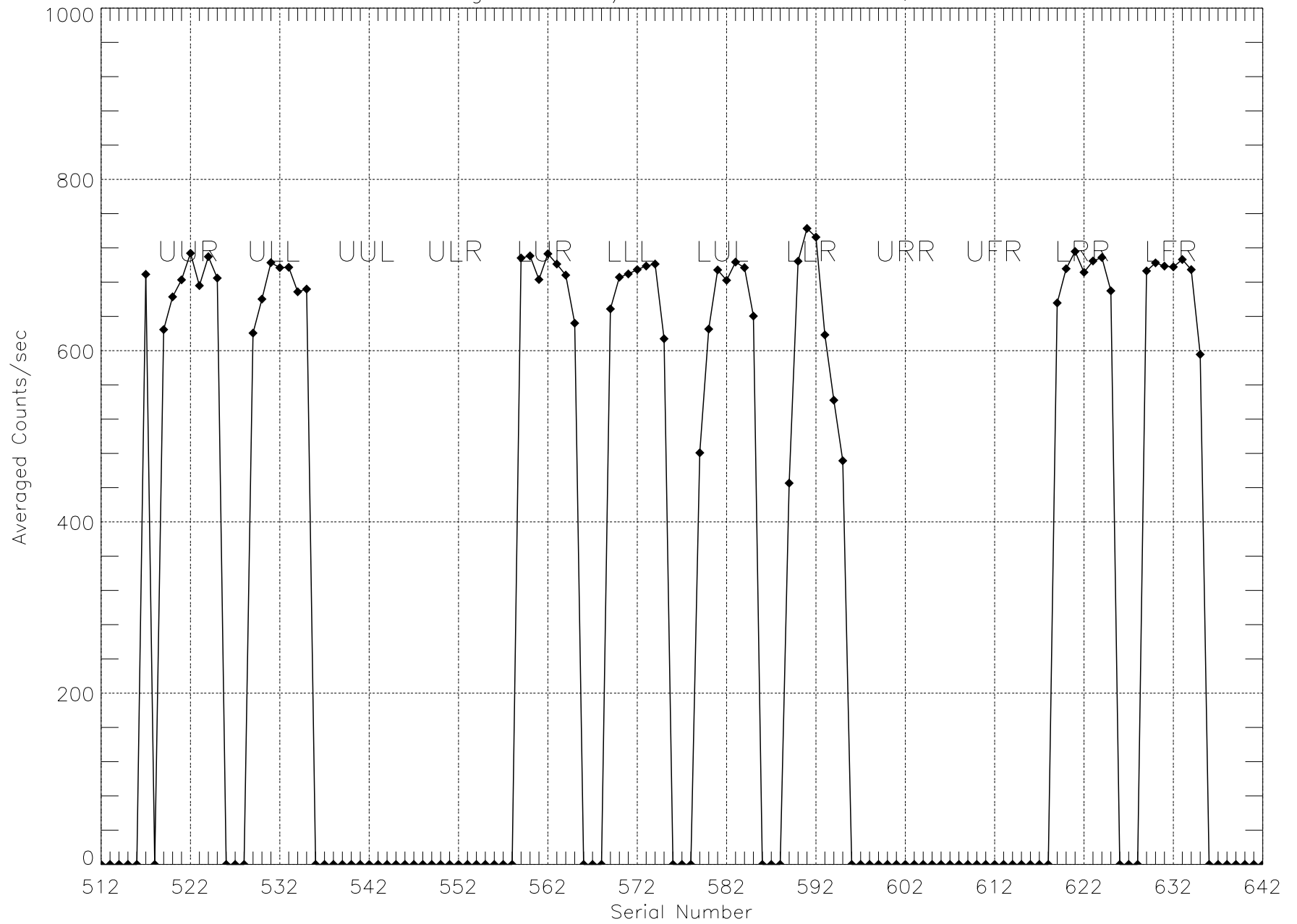
Averaged Counts/sec vs Serial Number, IS3
