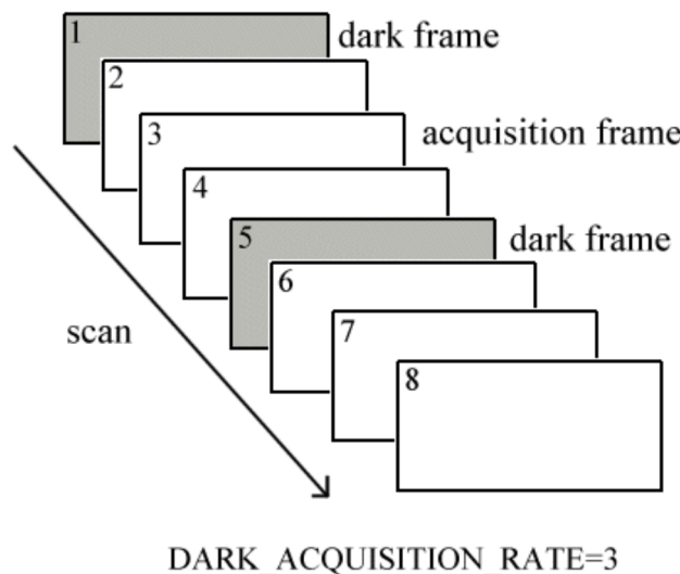
Figure 4-2: Structure of dark frames acquisition.
