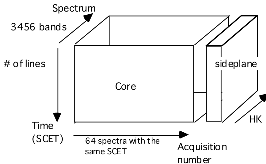
Figure 4-3: VIRTIS H data cube in 64-spectra mode. In this case, each frame contains the 64 spectra transferred together. The # of bands is equal to 3456.
