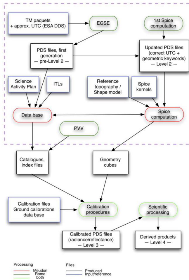
Figure 2-4: VIRTIS/Rosetta data set generation.
