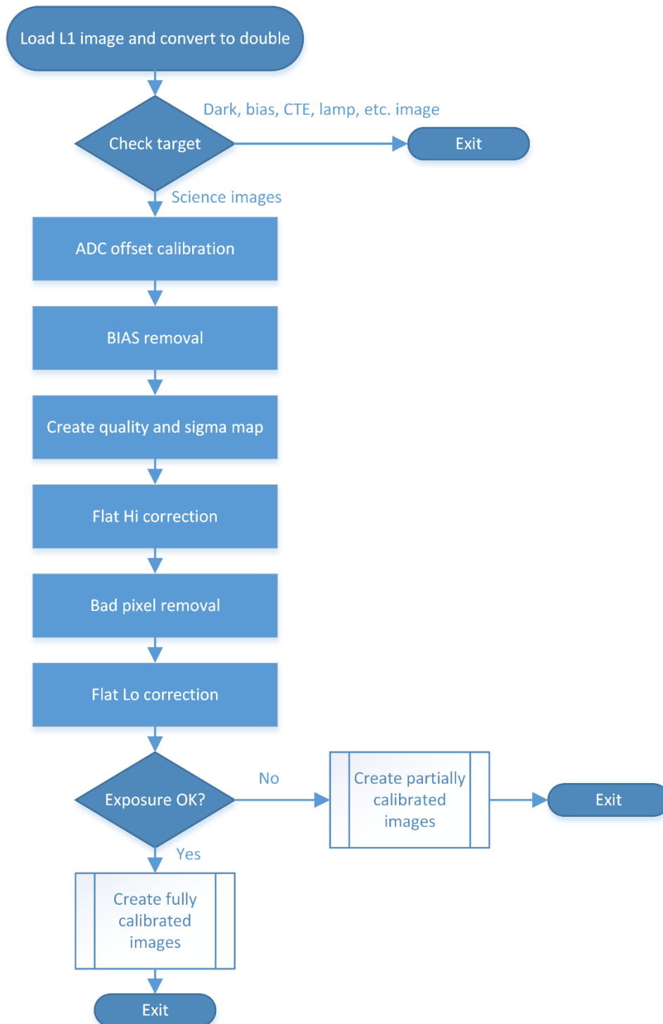
Figure 4 OsiCalliope main image calibration algorithm
