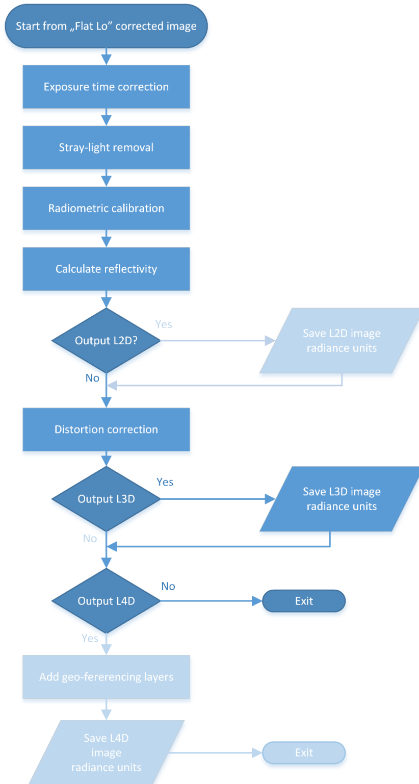
Figure 8 OSIRIS full calibration steps for solar stray-light corrected images in reflectance units
