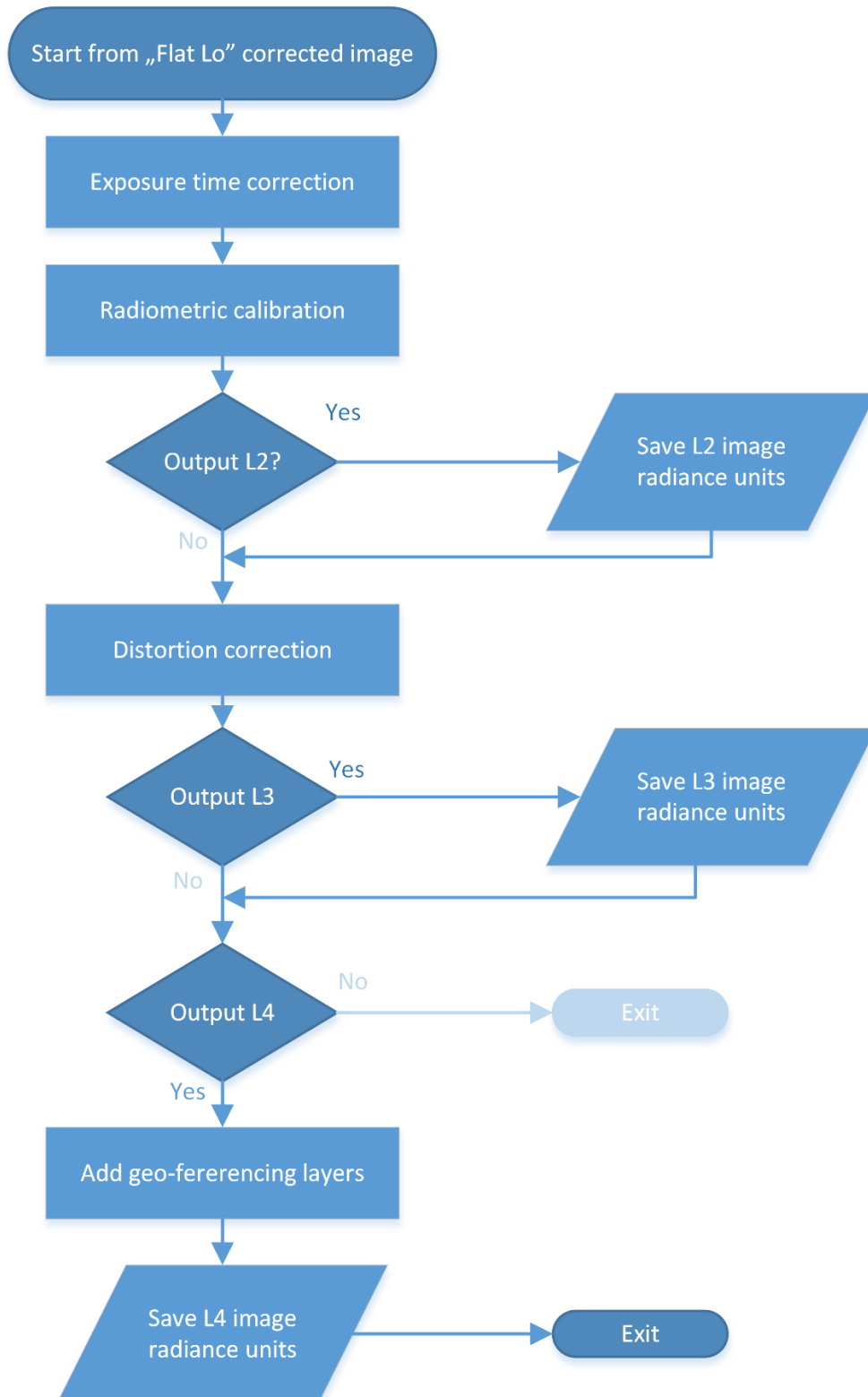
Figure 6 OSIRIS full calibration steps for images in radiance units
