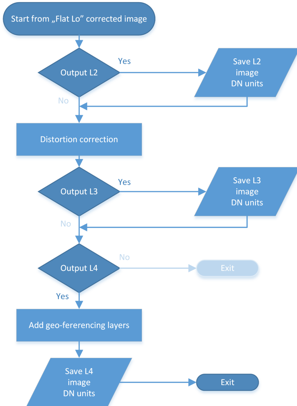
Figure 5 OSIRIS partial calibration steps – in case valid exposure time correction cannot be calculated.
