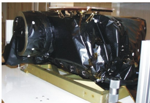
Figure 1: (left) The OSIRIS NAC flight unit in the lab. (right) The NAC Optical path
