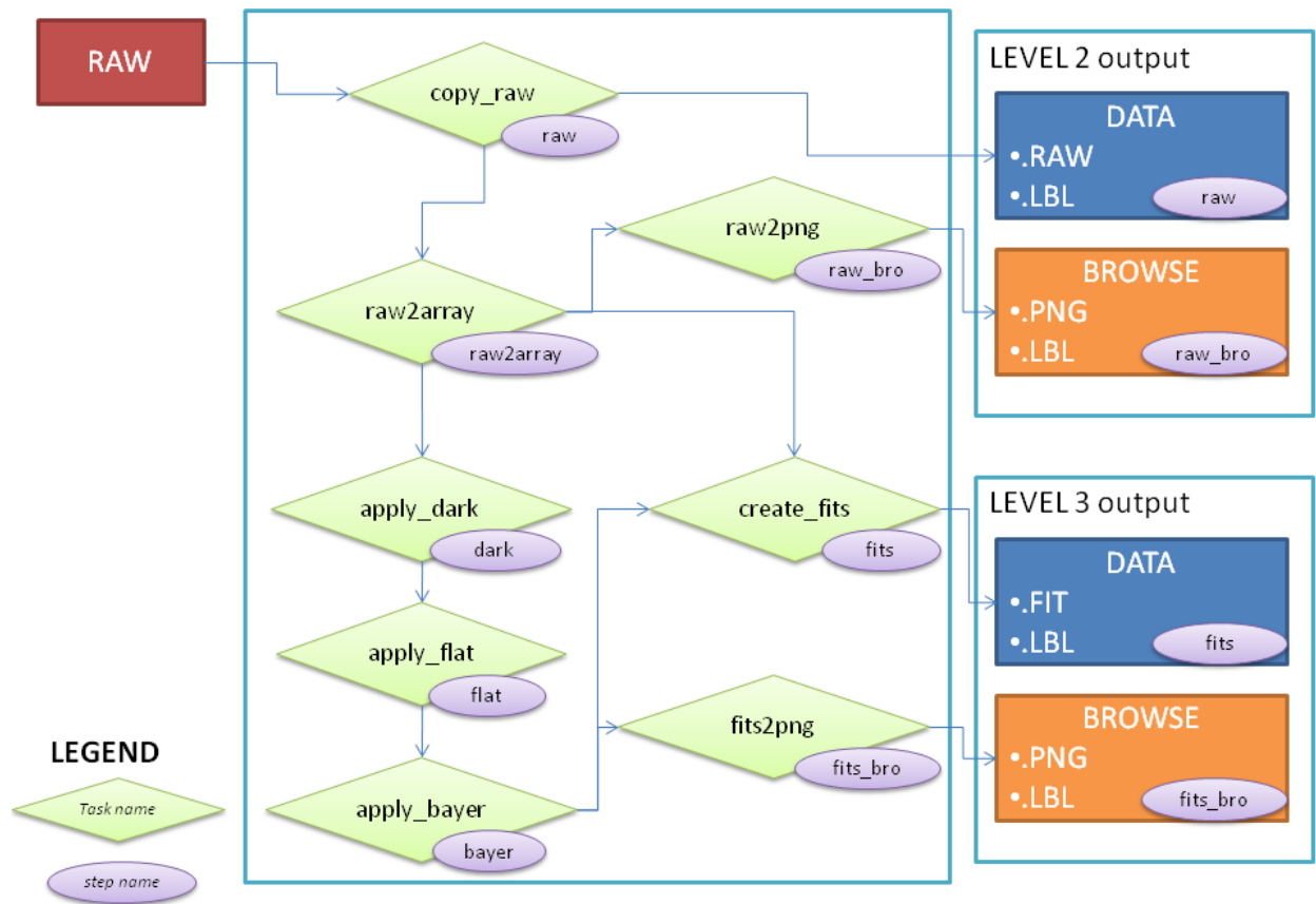
Figure 3: Flowchart of the full VMC data pipeline used to process raw and calibrated data products, as well as browse images.
