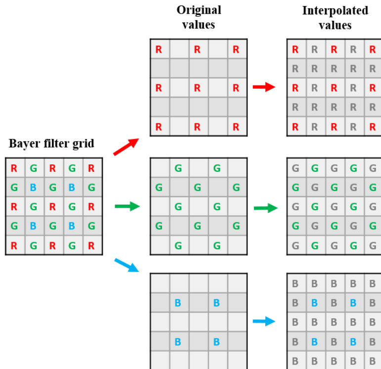
Figure 2: Debayering process. Coloured squares indicate pixels that keep their original value, grey boxes indicate where that colour channel is interpolated from the surrounding pixels.
