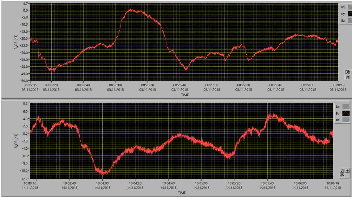
Figure 2: Examples of not visible WOL interference recorded on 03.11.2015 (top) and 14.11.2015 (bottom) during the ESC4 phase with the OB sensor. The x-axis shows time, the y-axis shows magnetic field components. Note that the scaling varies from panel to panel.
