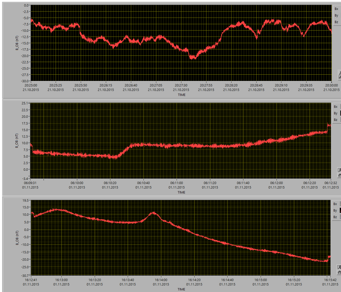
Figure 1: Examples of WOL disturbance recorded on 21.10.2015 (top), 01.11.2015 (center, bottom) during the ESC4 phase with the OB sensor. The x-axis shows time, the y-axis shows magnetic field components. Note that the scaling varies from panel to panel.
