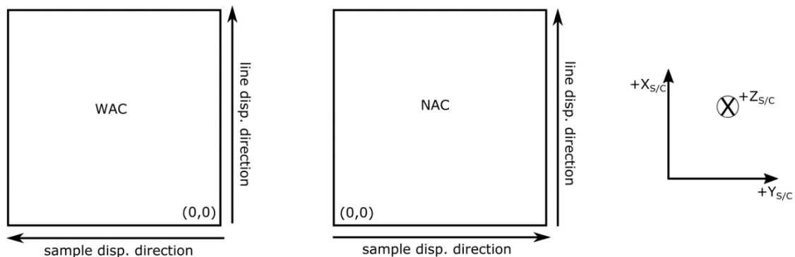
Figure 5: WAC and NAC images rotated into standard Rosetta orientation
