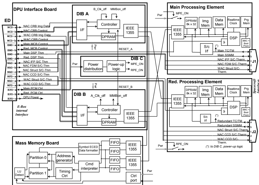
Figure 26. Block diagram of the OSIRIS DPU architecture.
