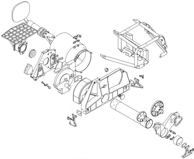
Figure 8. The NAC assembly. Focal plane and front door are on the upper left, primary and tertiary mirrors on the lower right.
