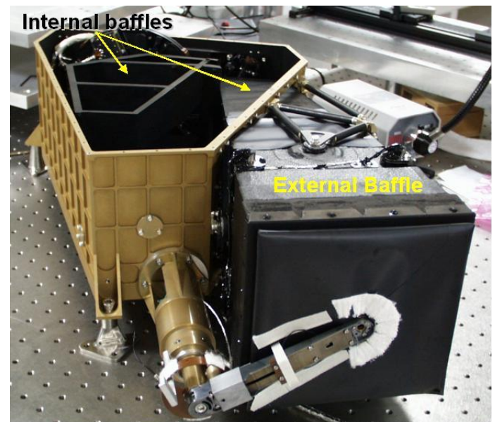
Figure 14. Concept and view of the WAC baffle.
