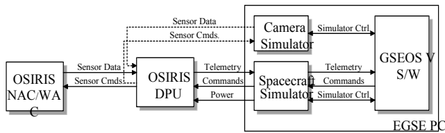
Figure 35. Commanding concept for the OSIRIS EGSE.
