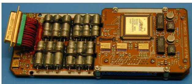
Figure 20. Shutter electronics board.
