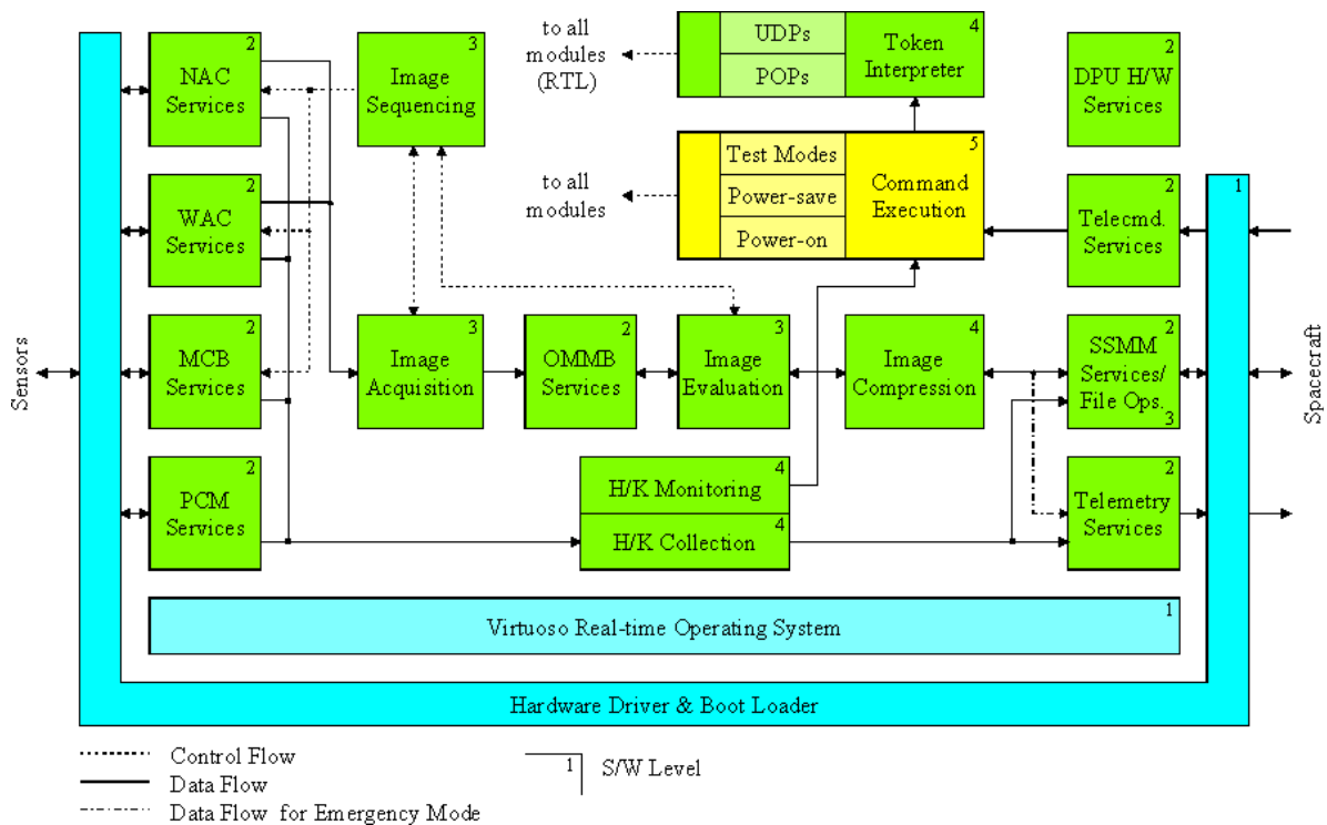
Figure 34. Interaction between software modules within OSIRIS.
