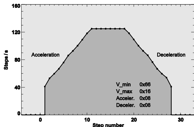
Figure 29. Nominal ramping of the motor step frequency.
