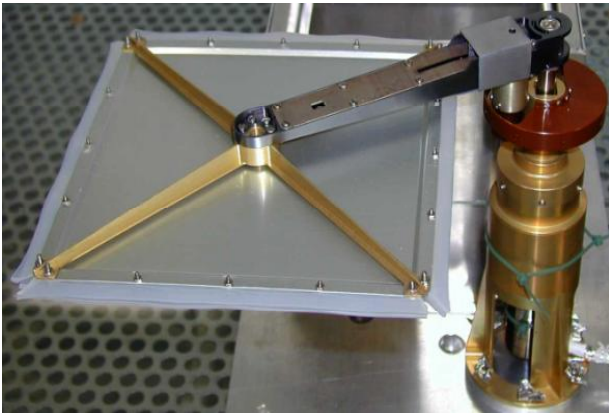
Figure 21. The integrated Front Door Mechanism.
