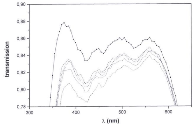
Figure 15. Transmission curves for irradiated KG3 glass. The bold curve provides the transmission prior to irradiation. The dashed curves show the transmission at different times after irradiation with subsequent annealing.
