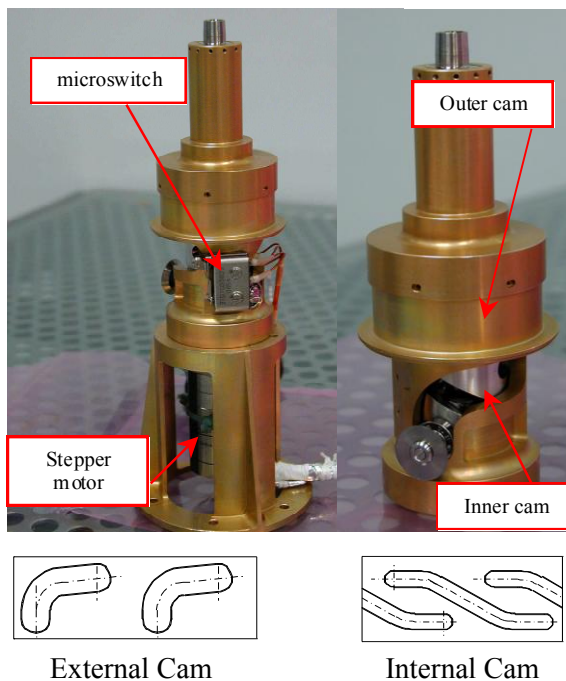
Figure 19. Components of the FDM and cylindrical development of the cams.
