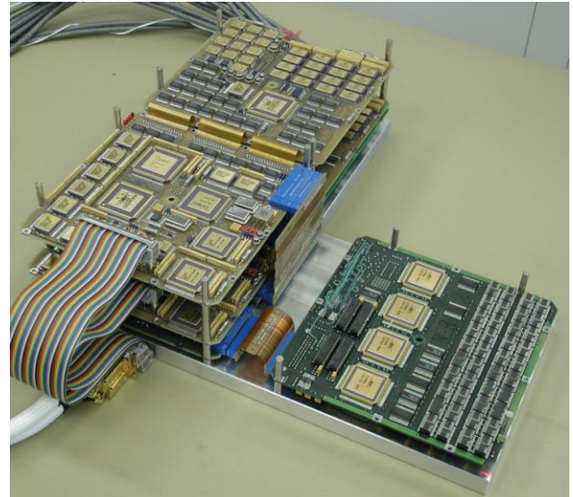
Figure 27. DPU FM under test with a prototype of the Mass Memory Board.
