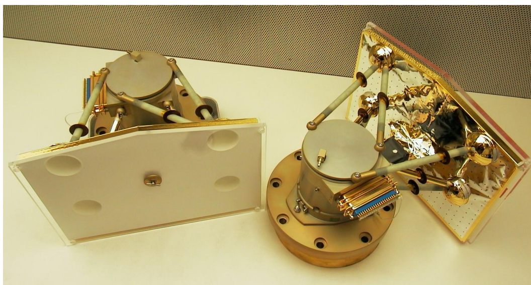
Figure 25. NAC and WAC Focal Plane Assembly.
