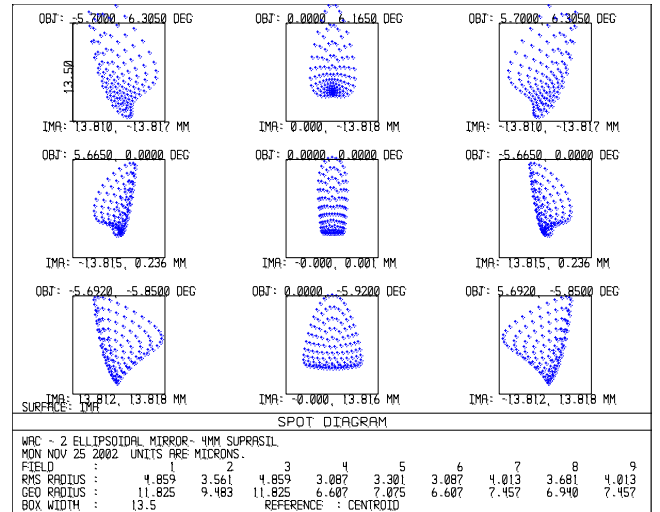
Figure 12. WAC spot diagram. The spots refer to the centre, the edges and the corners of the 12°×12° FOV. The boxes correspond to the pixel size of the detector.
