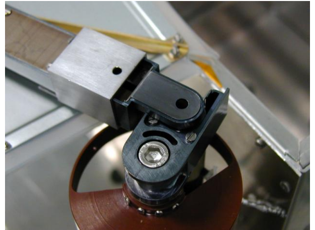
Figure 22. Activated fail-safe device of the Front Door Mechanism.
