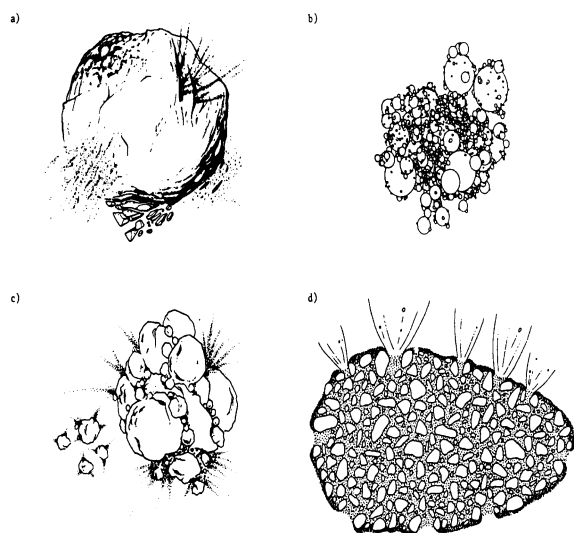
Figure 4. Conceptual models of the structure of the cometary nucleus:
