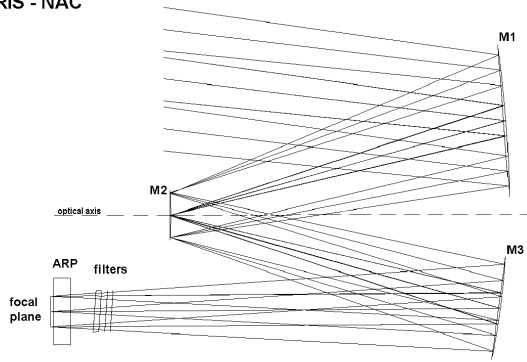
Figure 6. Ray paths through the NAC optical system.
