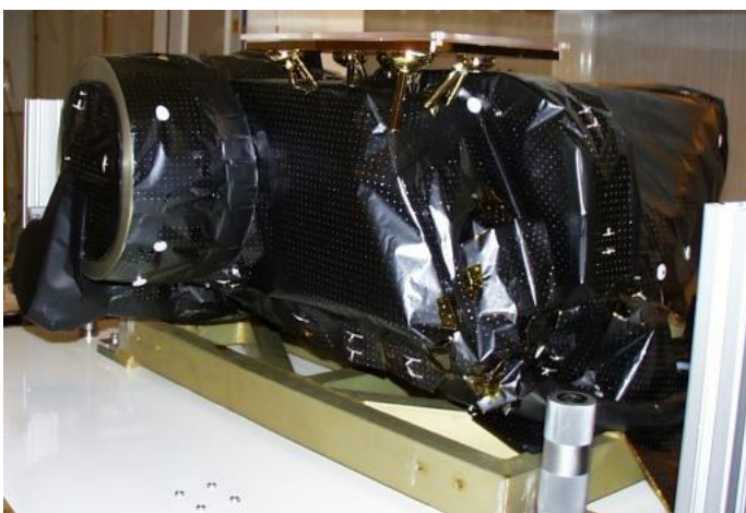
Figure 9. NAC Flight Model during integration and in flight configuration.
