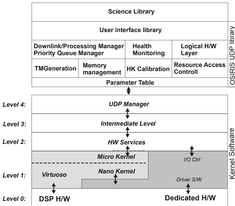
Figure 32. Structure of the OSIRIS flight software.
