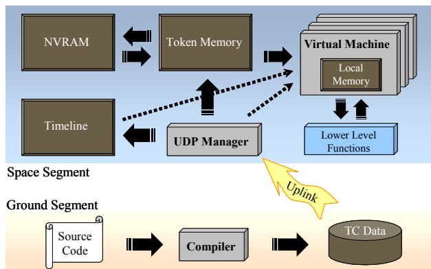
Figure 33. Architecture of the OSIRIS Command Language system.
