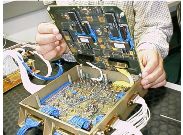
Figure 30. Bread-board model of the E-Box Power Converter Module.
