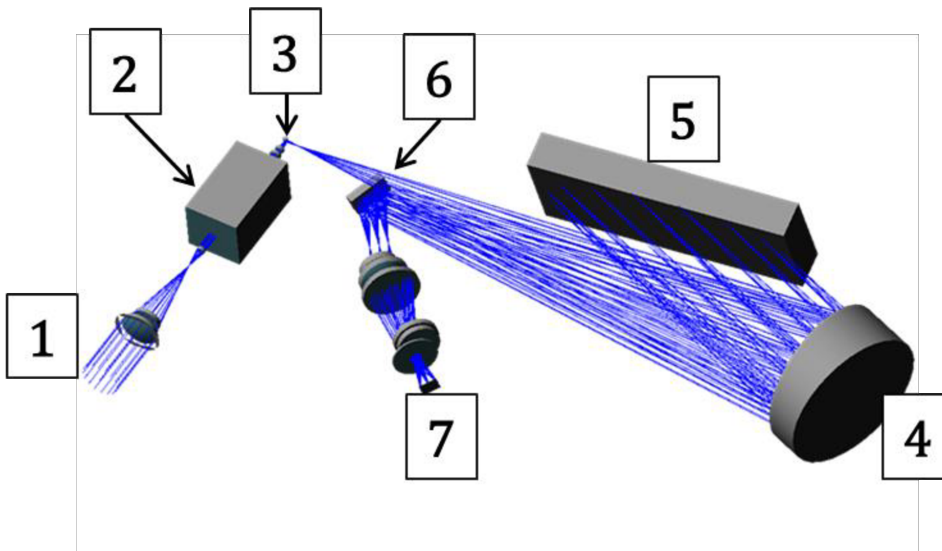
Figure 2: Schematics of the SO and LNO channels: (1) the entrance optics, (2) the AOTF filter, (3) the spectrometer entrance slit, (4 & 6) folding mirrors, (5) the echelle grating, (7) the detector. Image from Vandaele et al. (2015) [RDO6]
