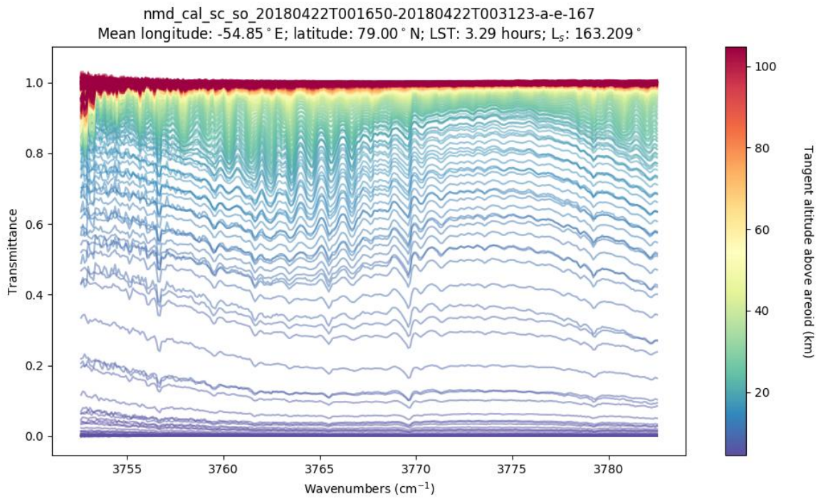
Figure 34: An example of an SO browse product, showing the signal versus altitude for the accepted bins of one diffraction order. The colour denotes the tangent altitude above the Areoid model. Mean geometric parameters are given the title.
