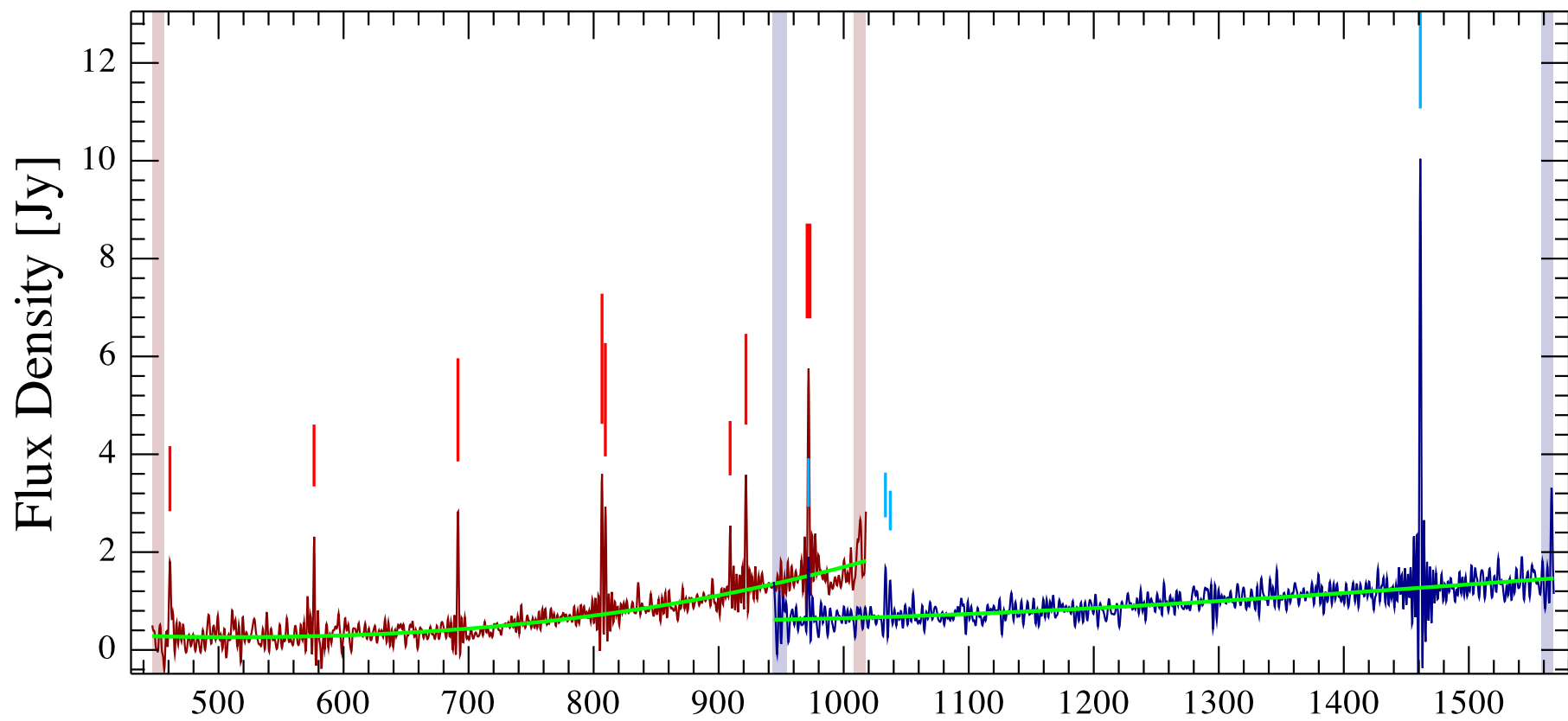
NGC 6853-offset-1 Observation ID 1342270195; (8/4)
