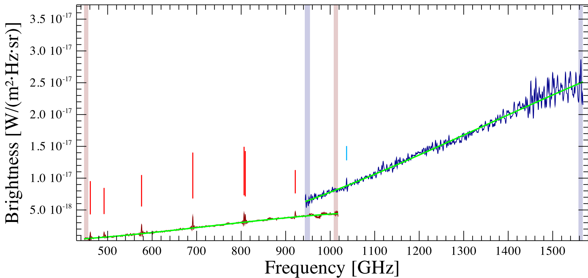
PDS 27 Observation ID 1342270035; (7/1)
