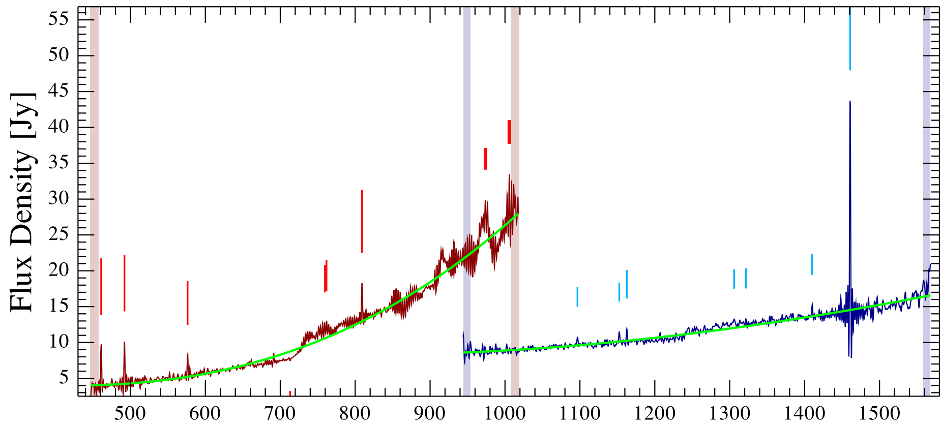
IRAS 18488-0107 Observation ID 1342268317; (7/3)
