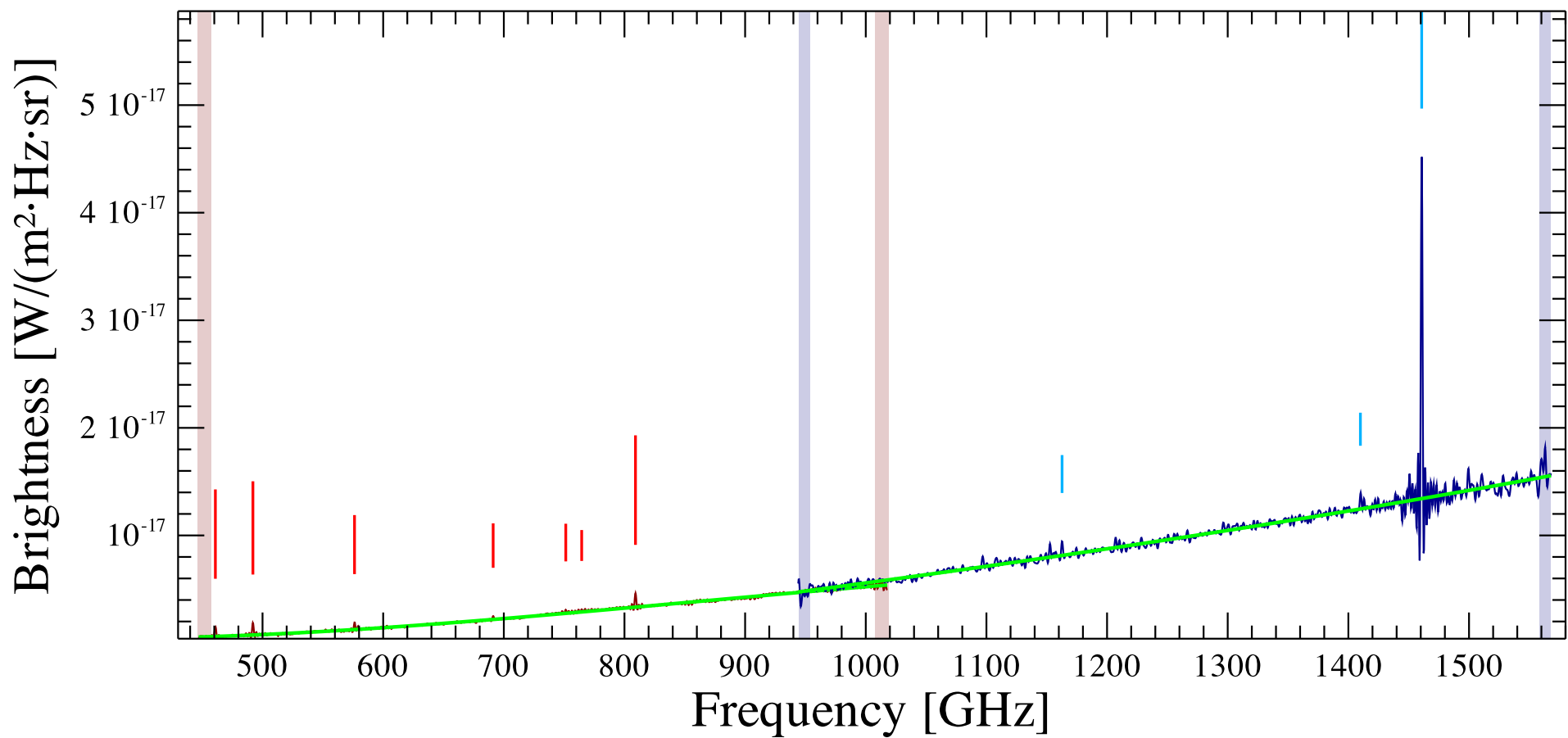
IRAS 18488-0107 Observation ID 1342268317; (7/3)
