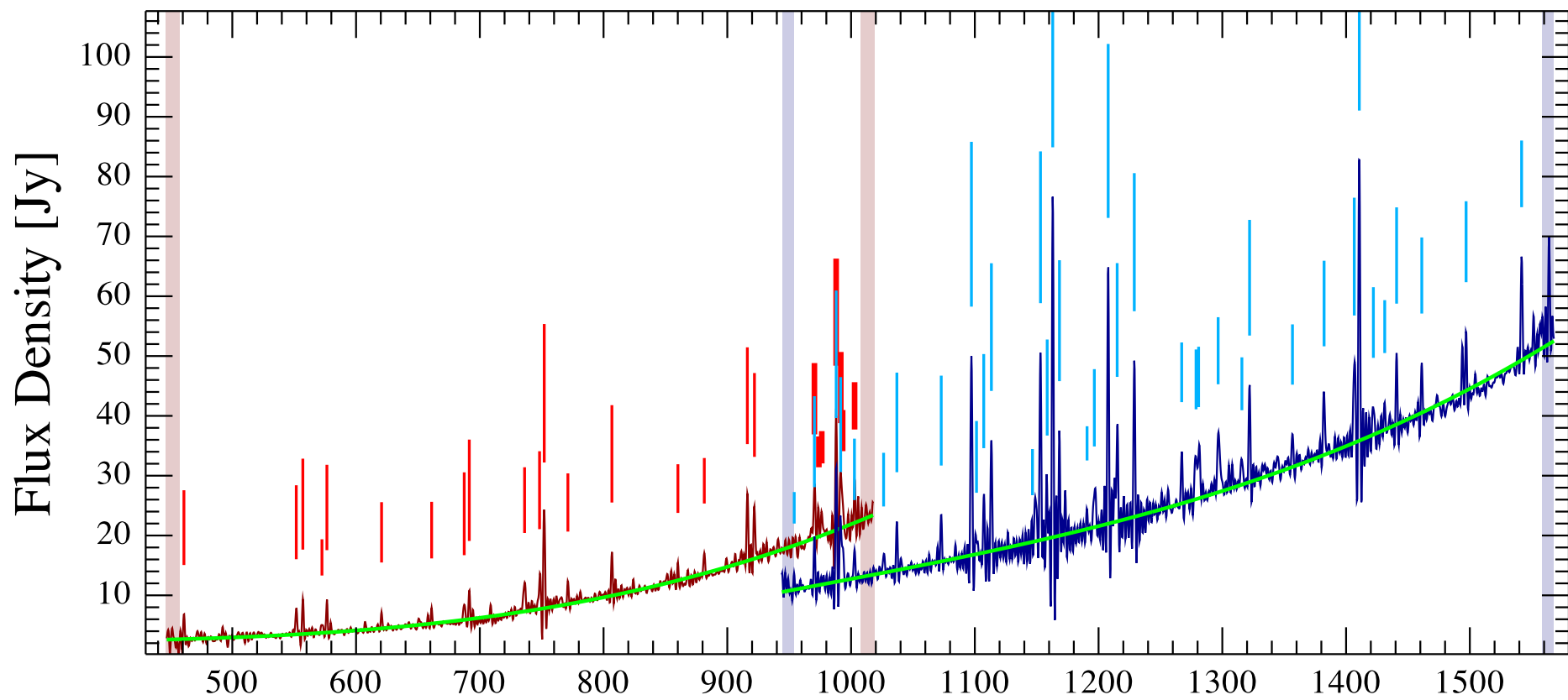
AFGL 5379 Observation ID 1342268287; (27/32)
