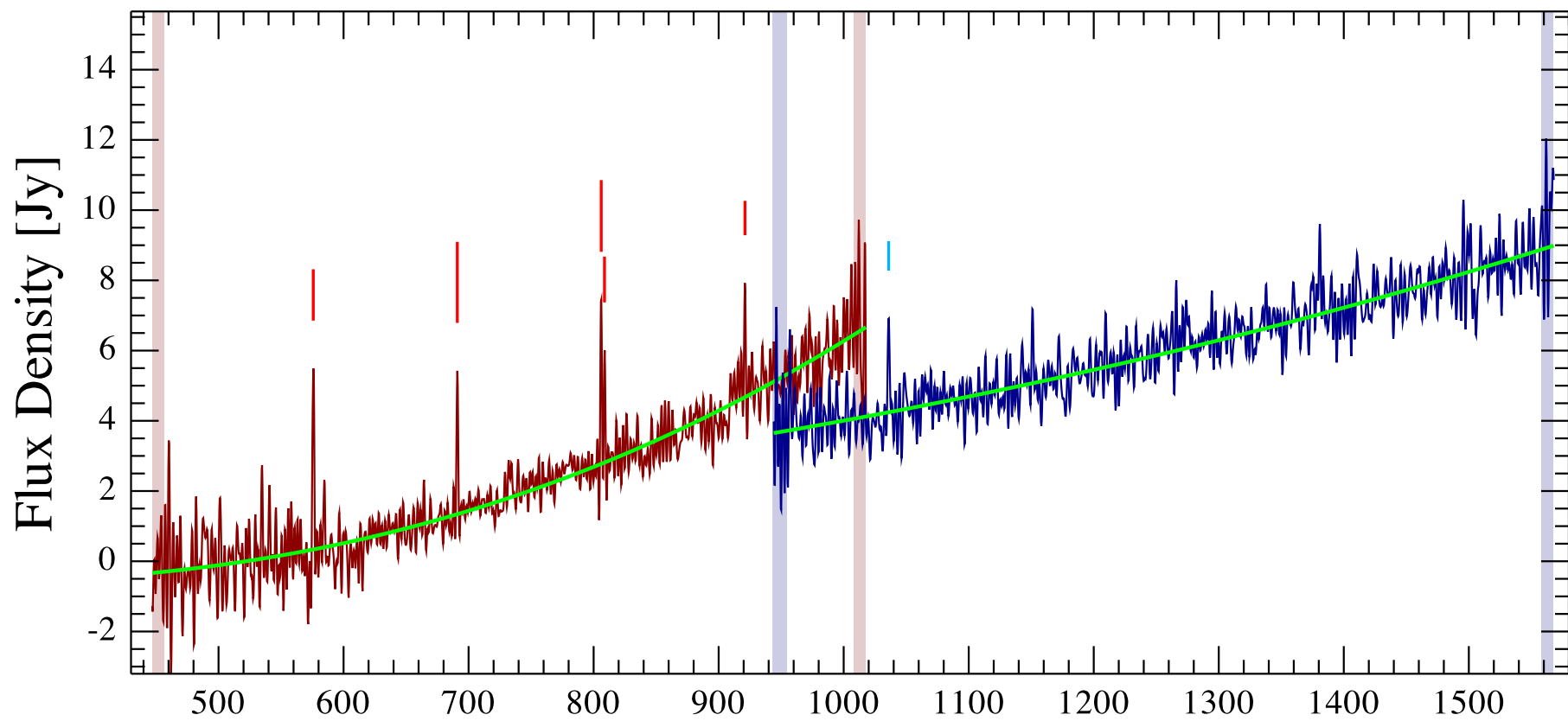
ST01 Observation ID 1342262910; (5/1)
