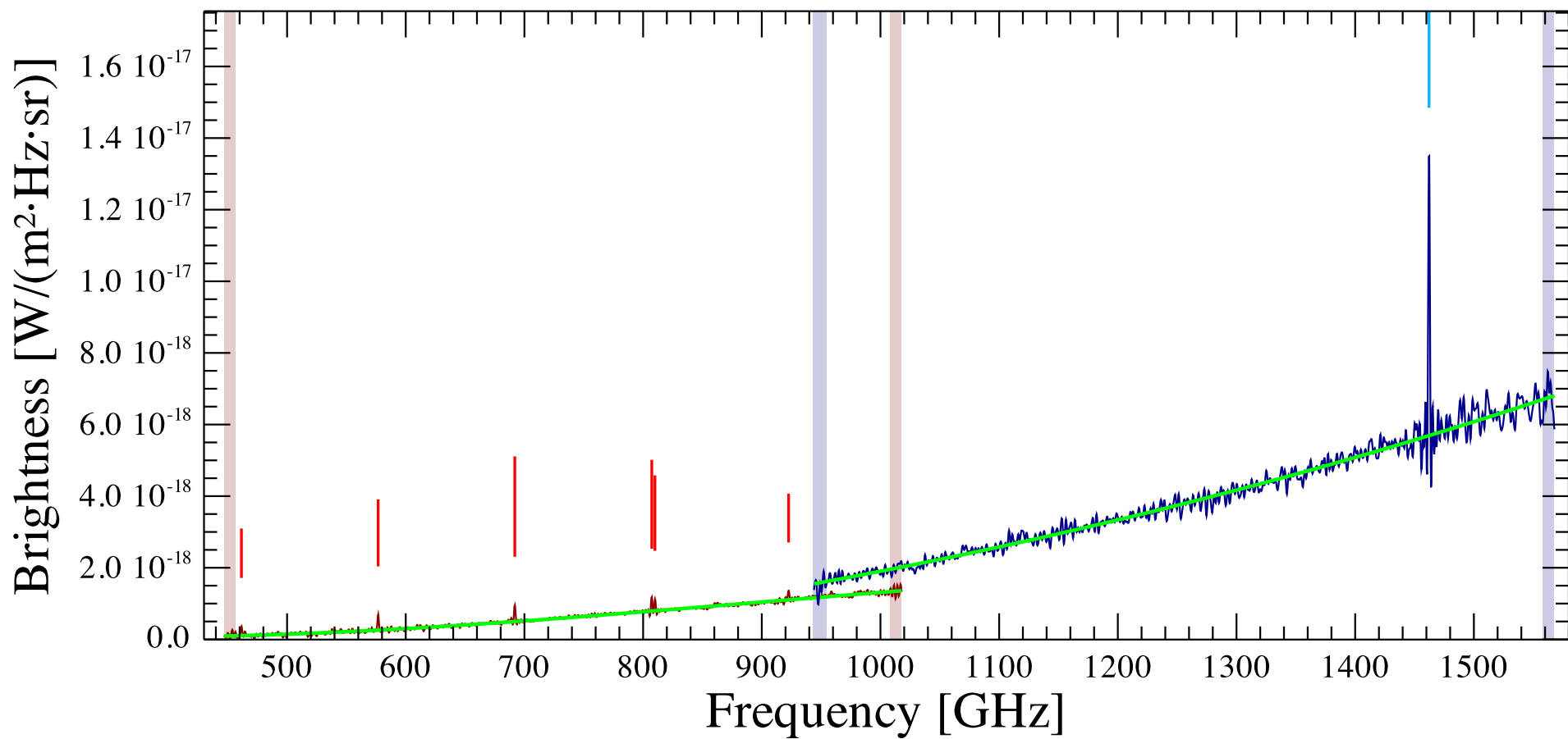
ngc604gmc2 Observation ID 1342259067; (6/1)
