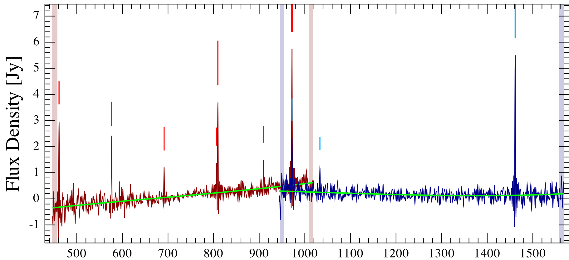
NGC 7293 Observation ID 1342257353; (7/3)
