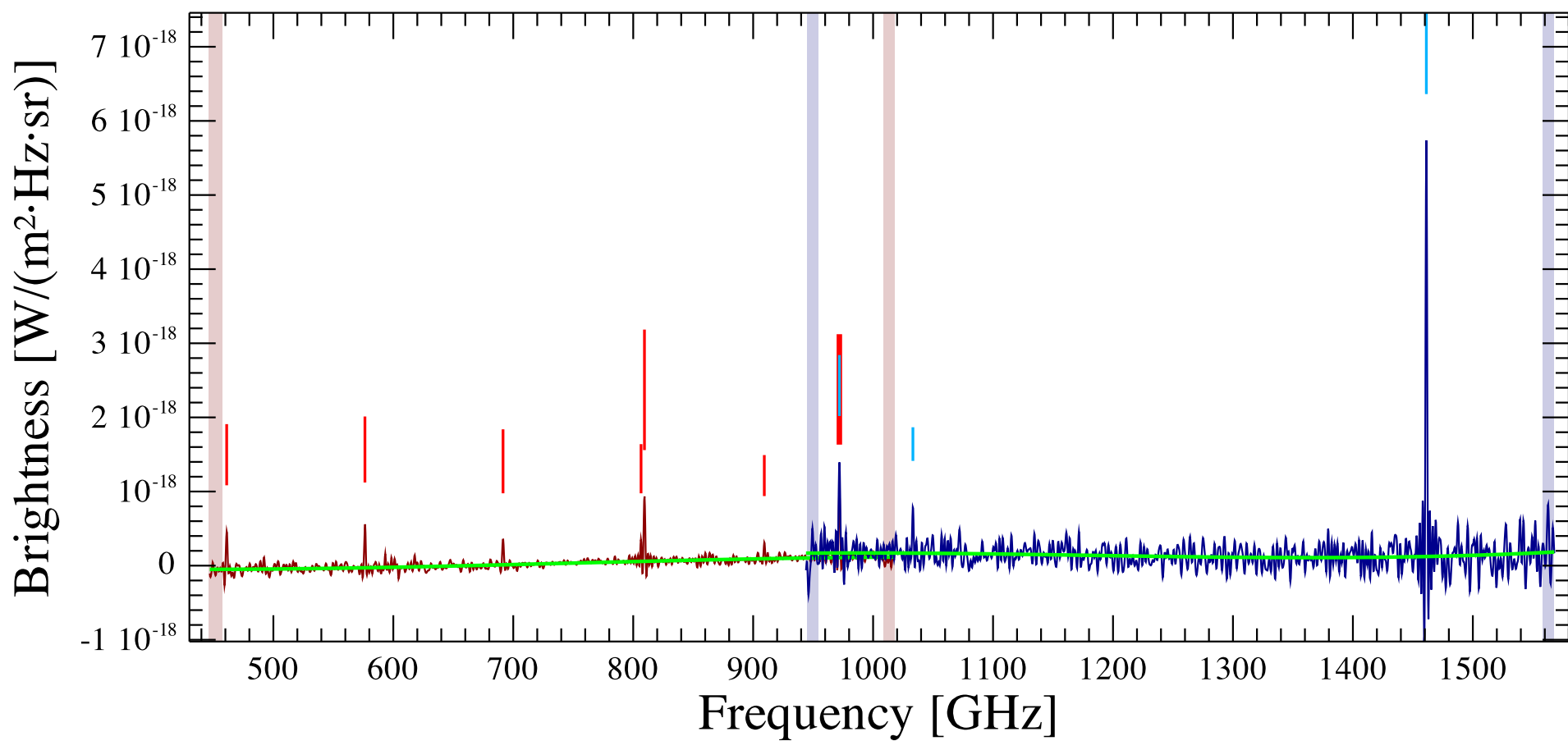
NGC 7293 Observation ID 1342257353; (7/3)
