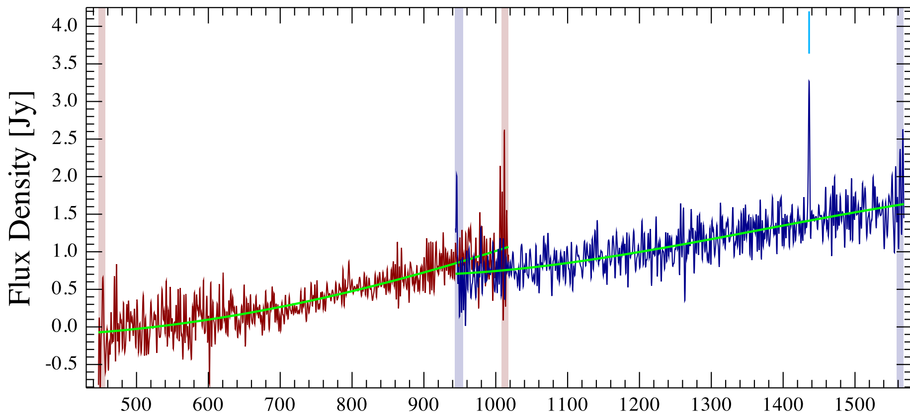
hcg 100a-1 Observation ID 1342257343; (0/1)
