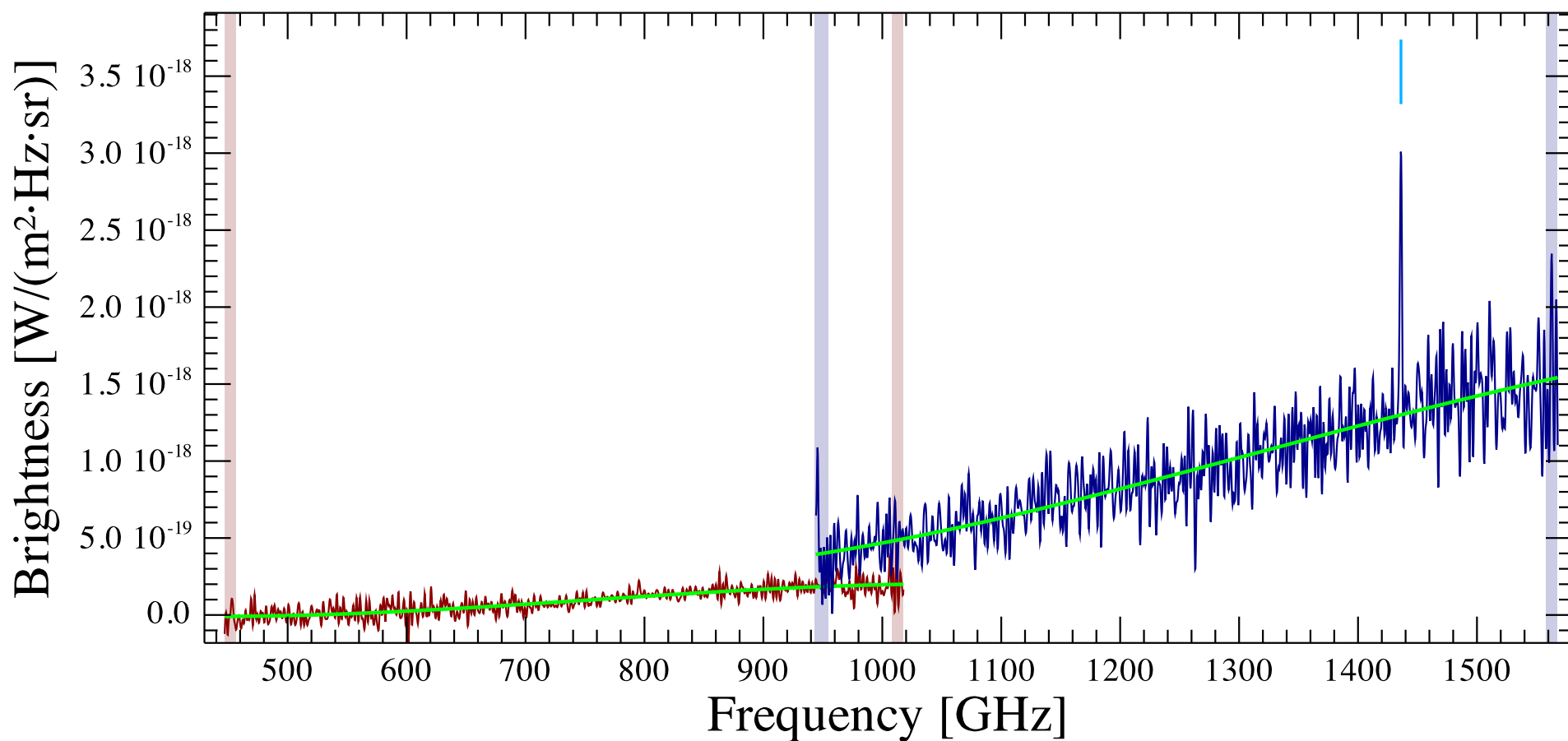
hcg 100a-1 Observation ID 1342257343; (0/1)
