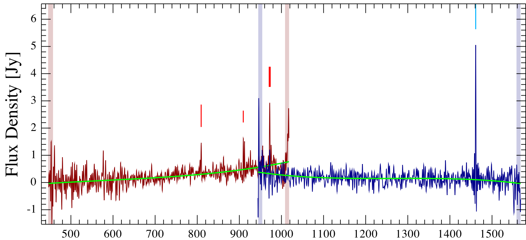
Helix T2 Observation ID 1342256099; (3/1)
