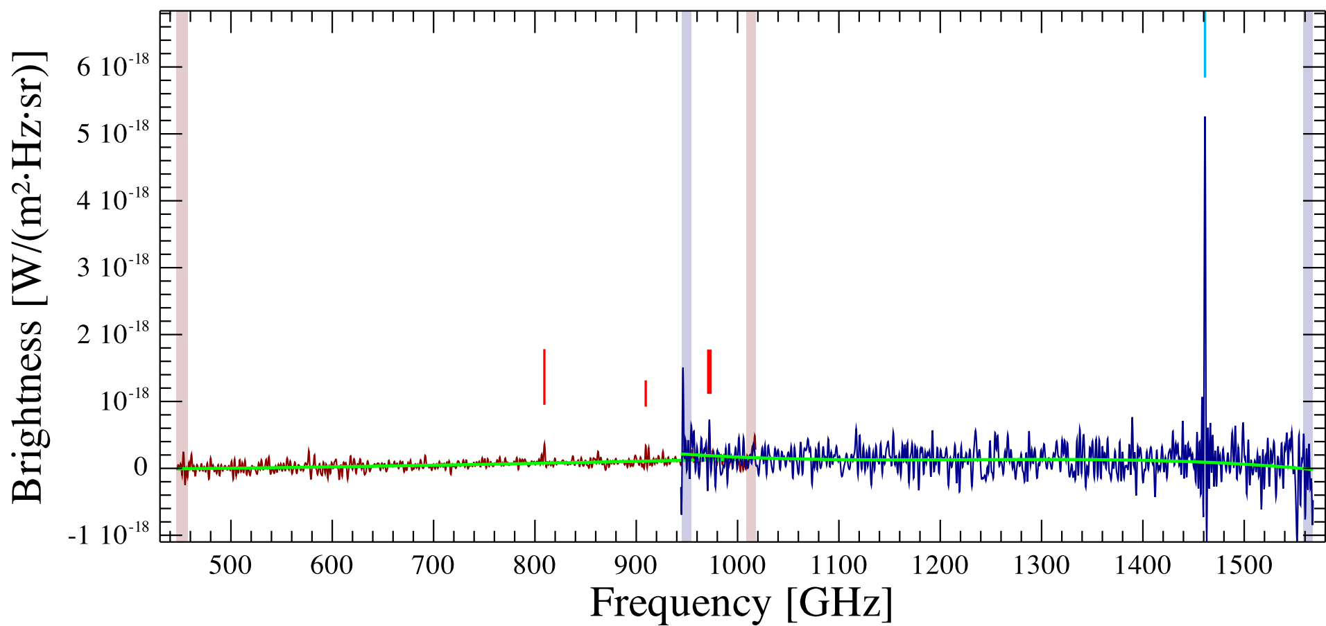
Helix T2 Observation ID 1342256099; (3/1)
