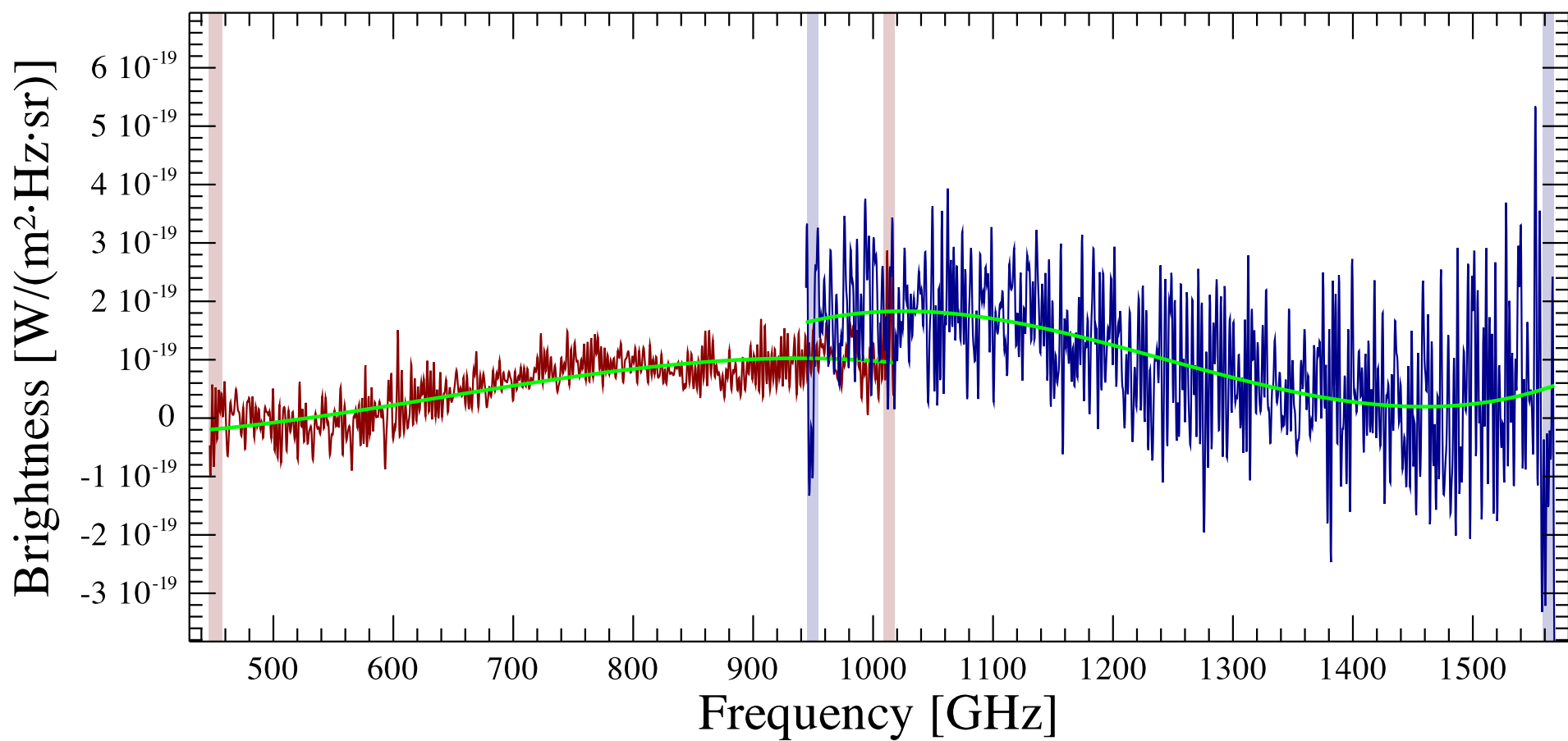
MM1842 Observation ID 1342255811; (0/0)
