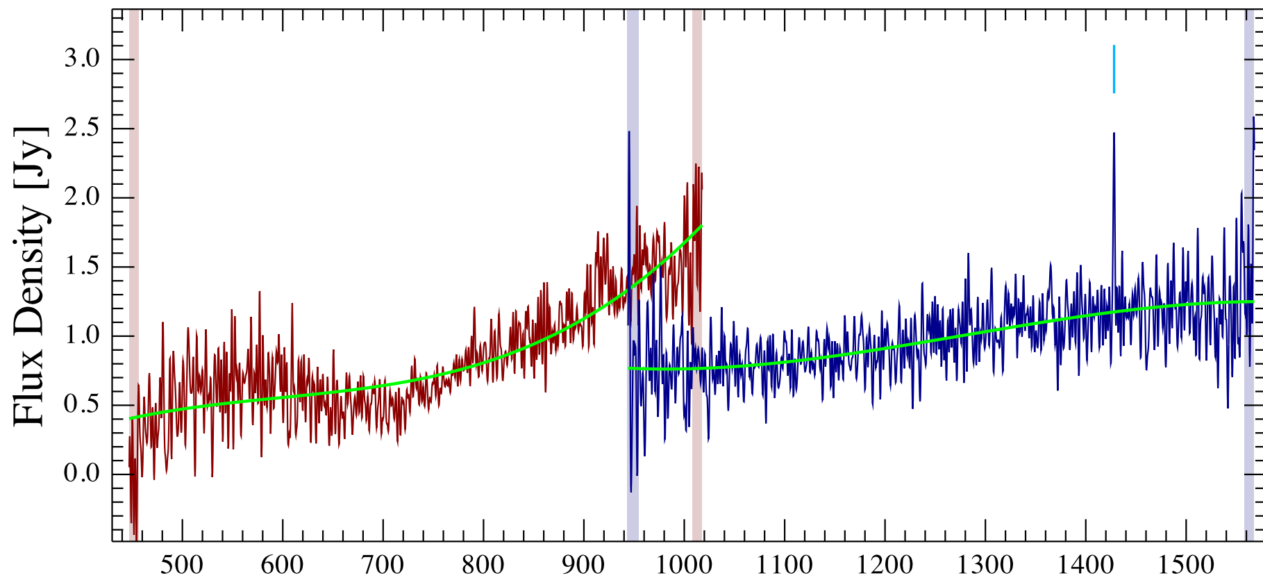
hcg 91a-1 Observation ID 1342255264; (0/1)
