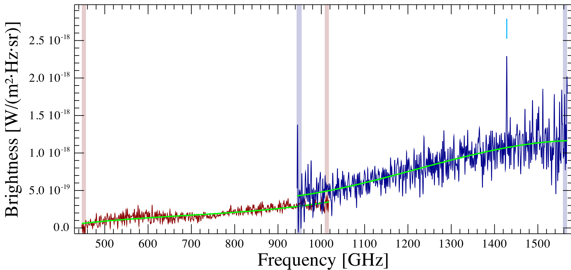
hcg 91a-1 Observation ID 1342255264; (0/1)
