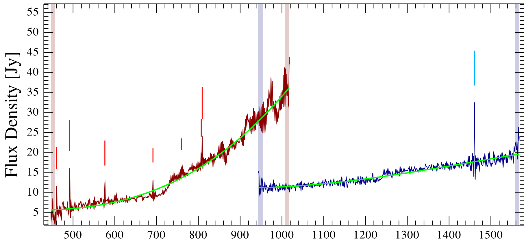
MGE_3681 Observation ID 1342253970; (7/1)
