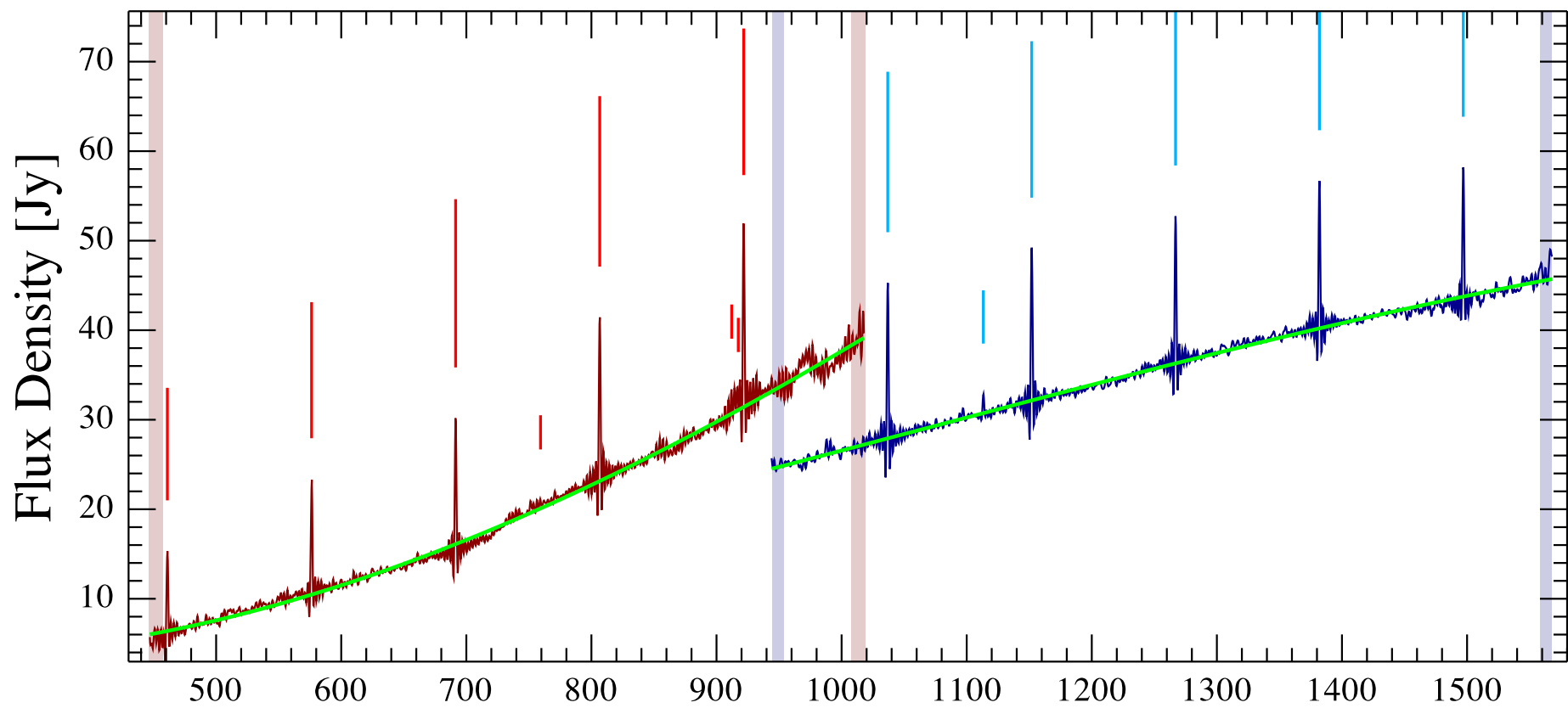
B335 Observation ID 1342253652; (5/10)
