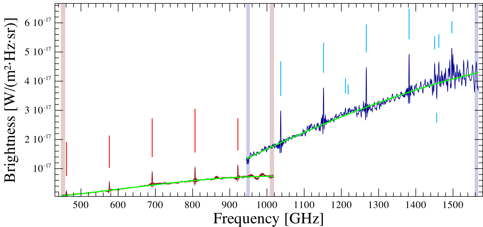
B335 Observation ID 1342253652; (5/10)
