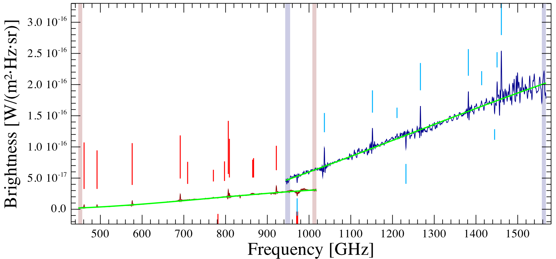
G24.94+0.07 Observation ID 1342252901; (14/11)
