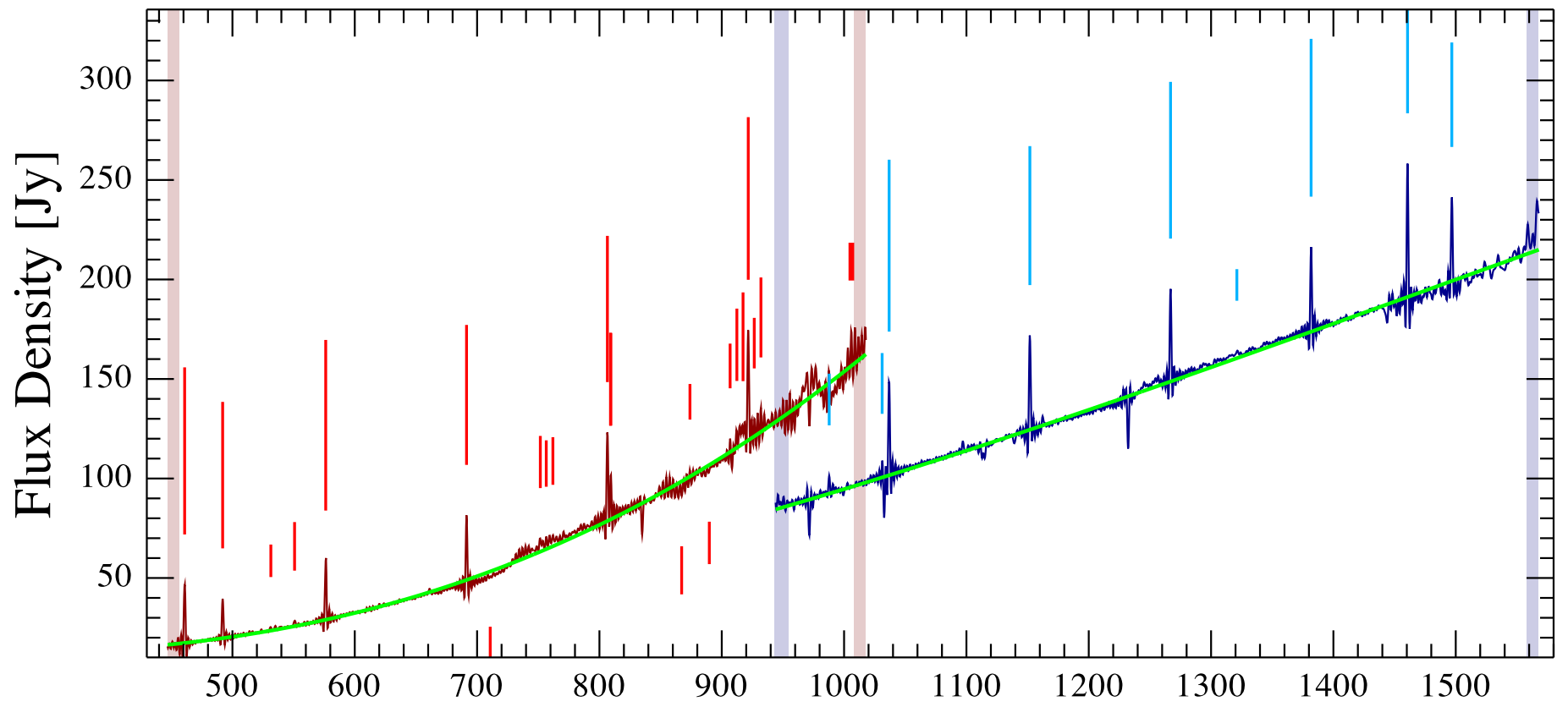
G24.94+0.07 Observation ID 1342252901; (14/11)
