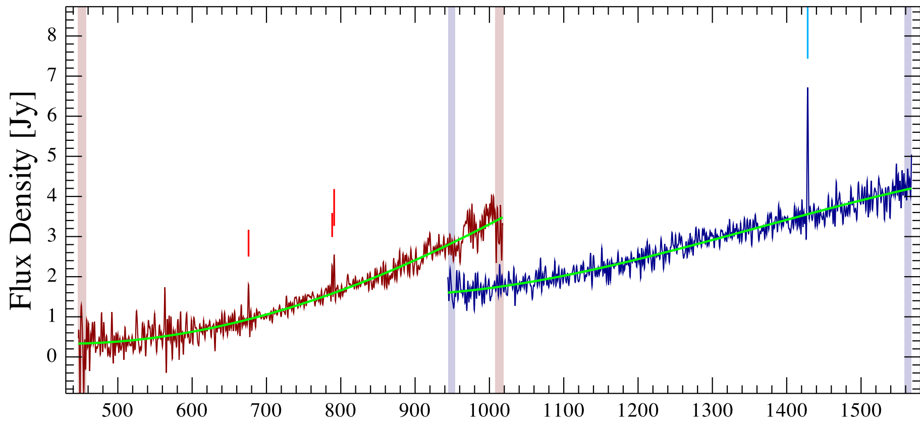
IRASF16516-0948 Observation ID 1342251335; (3/1)
