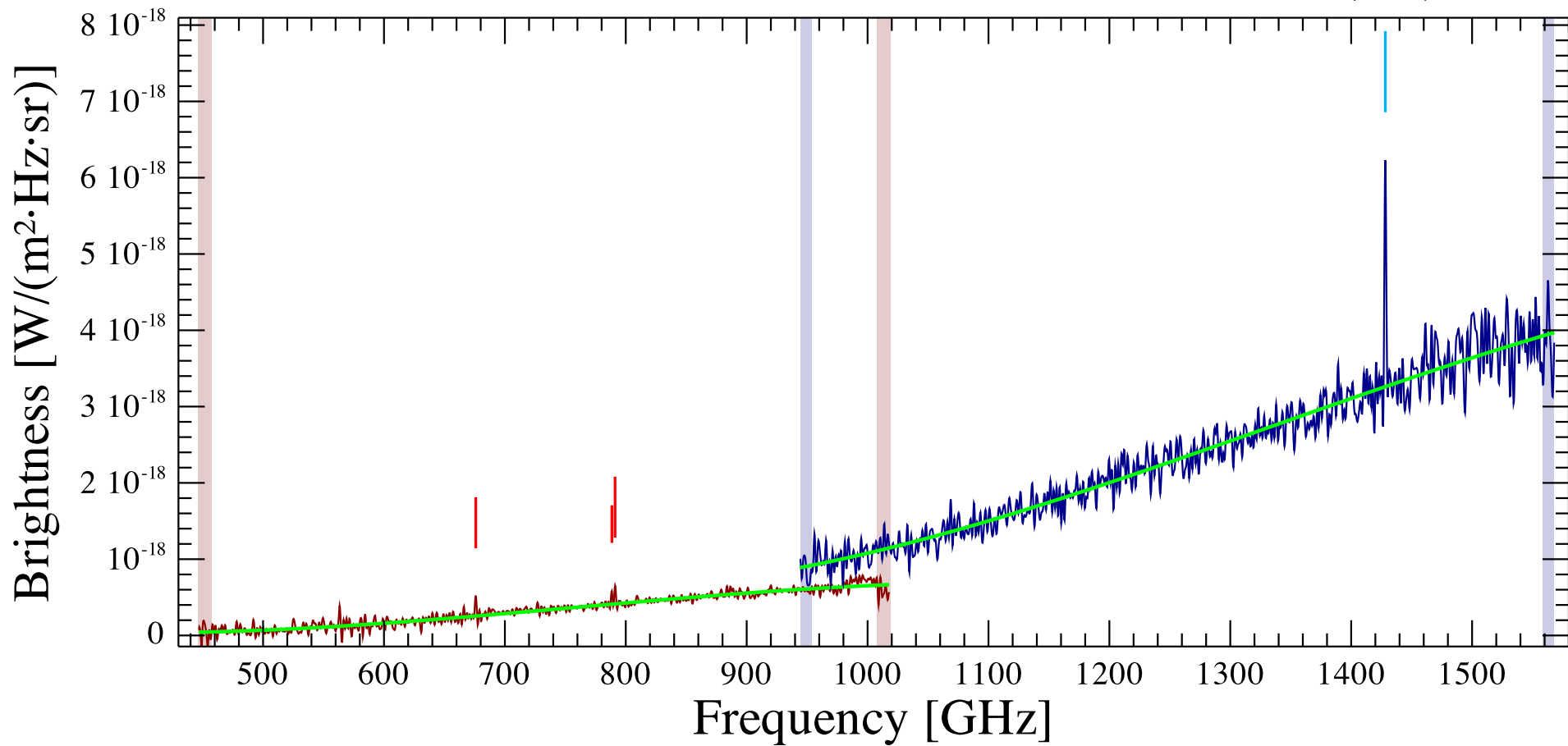
IRASF16516-0948 Observation ID 1342251335; (3/1)
