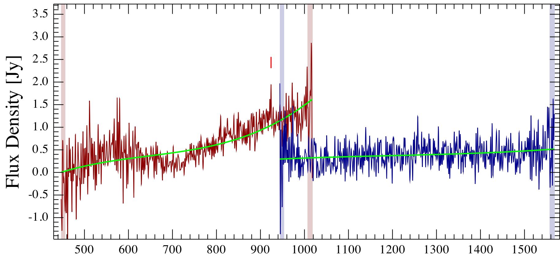
CB68 Observation ID 1342251332; (0/0)
