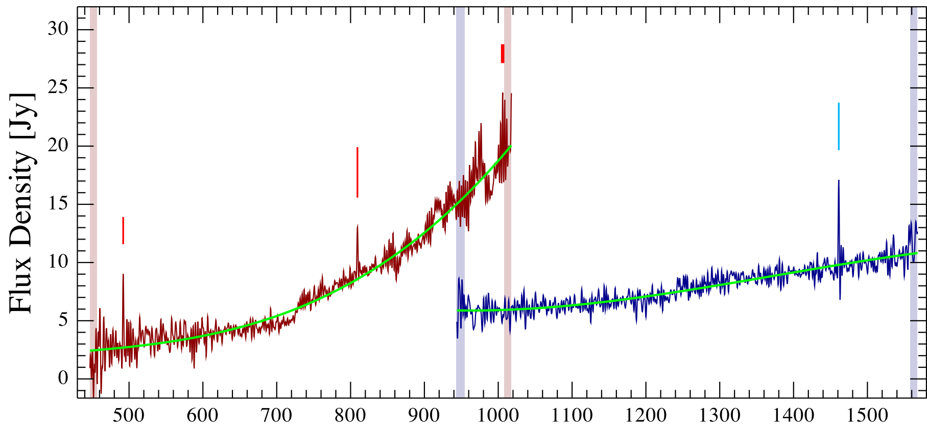
G357.7 ref Observation ID 1342251327; (2/1)
