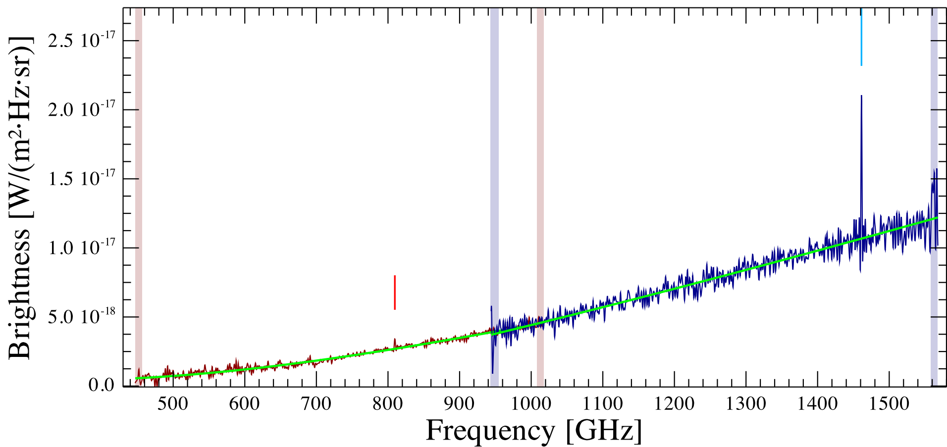
G349.7 ref Observation ID 1342251324; (1/1)
