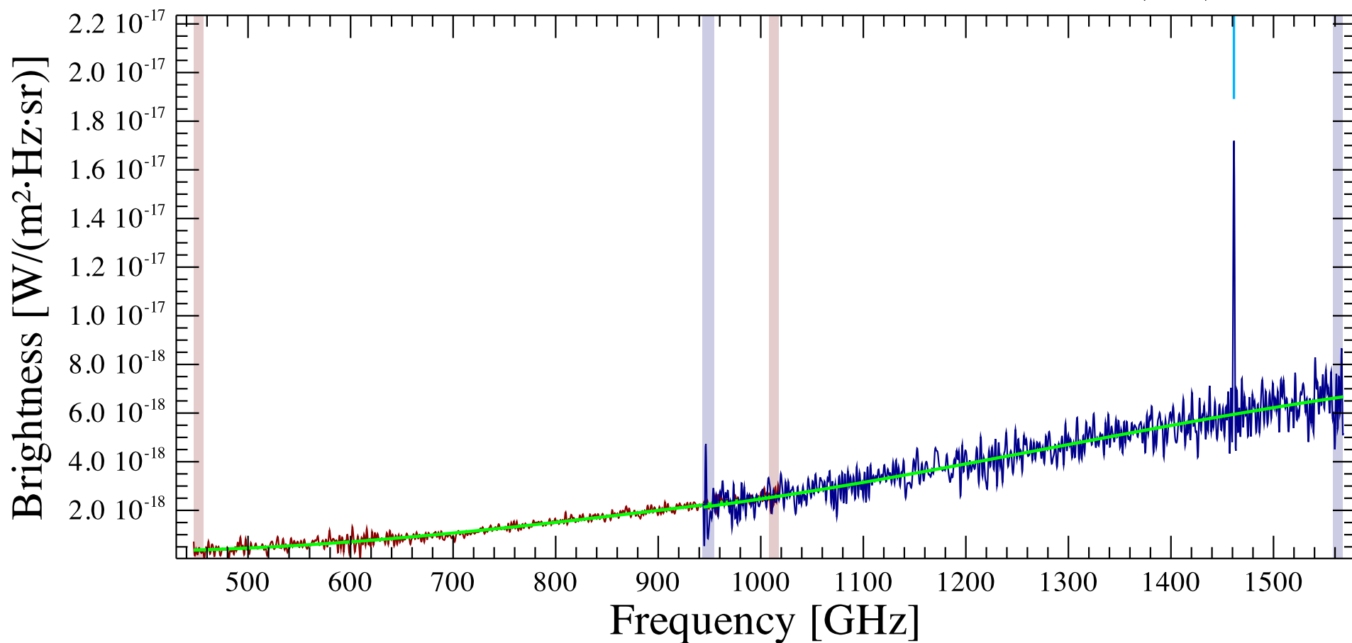
CTB37A-N ref Observation ID 1342251320; (0/1)
