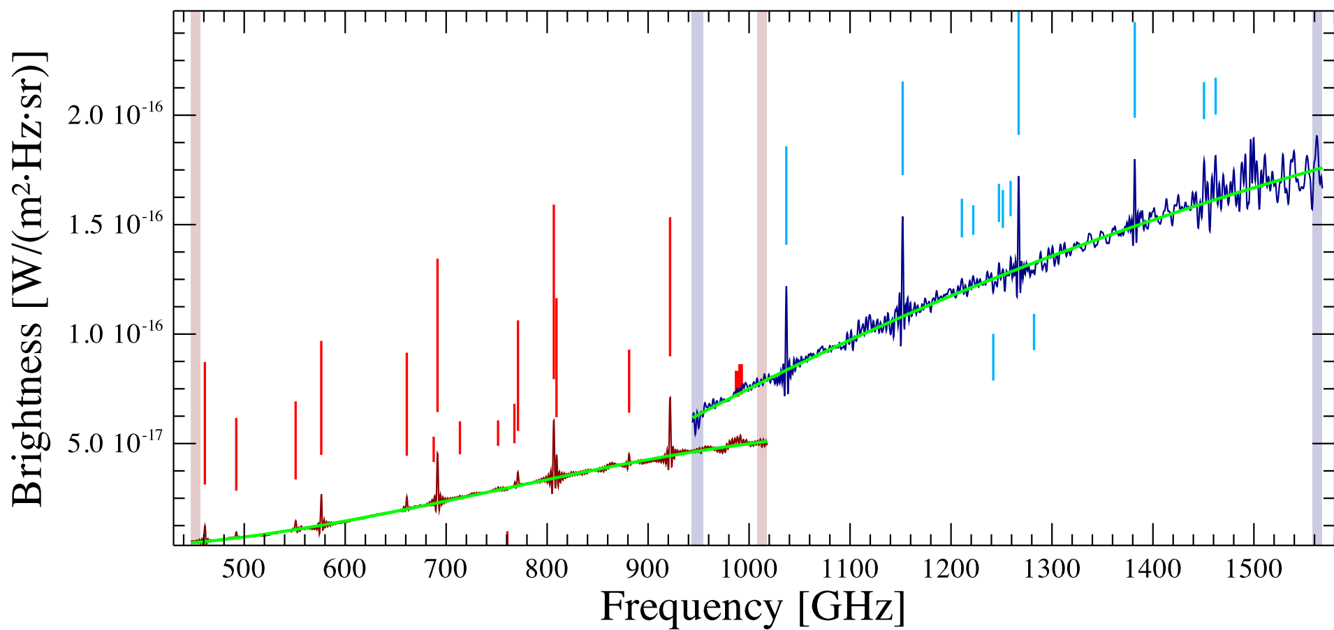
VLA 1623 Observation ID 1342251287; (18/13)
