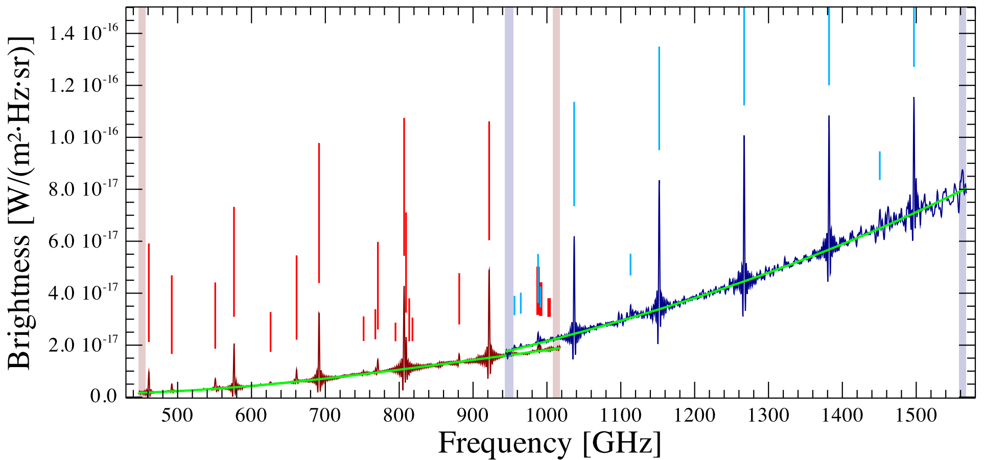
GSS 30 IRS1 Observation ID 1342251286; (20/11)
