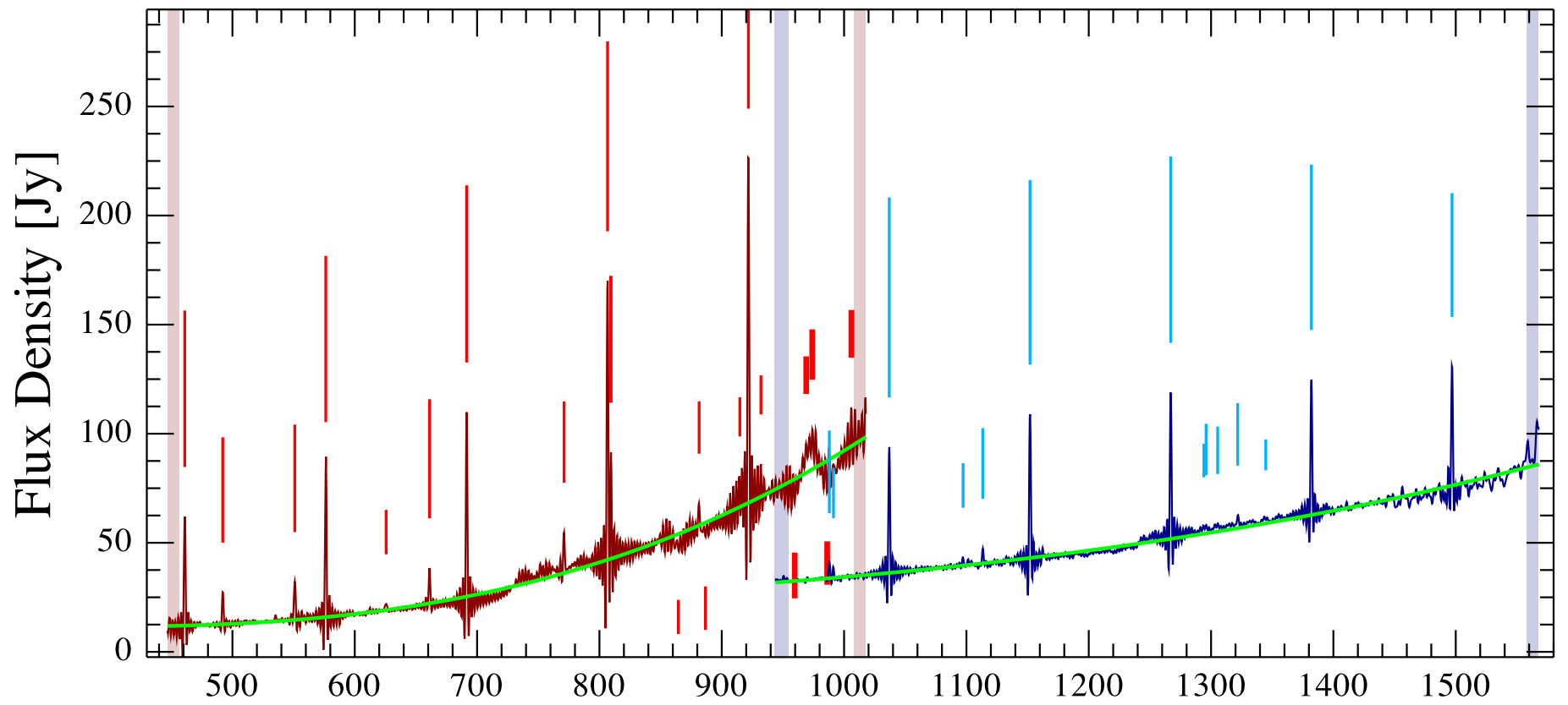
GSS 30 IRS1 Observation ID 1342251286; (20/11)
