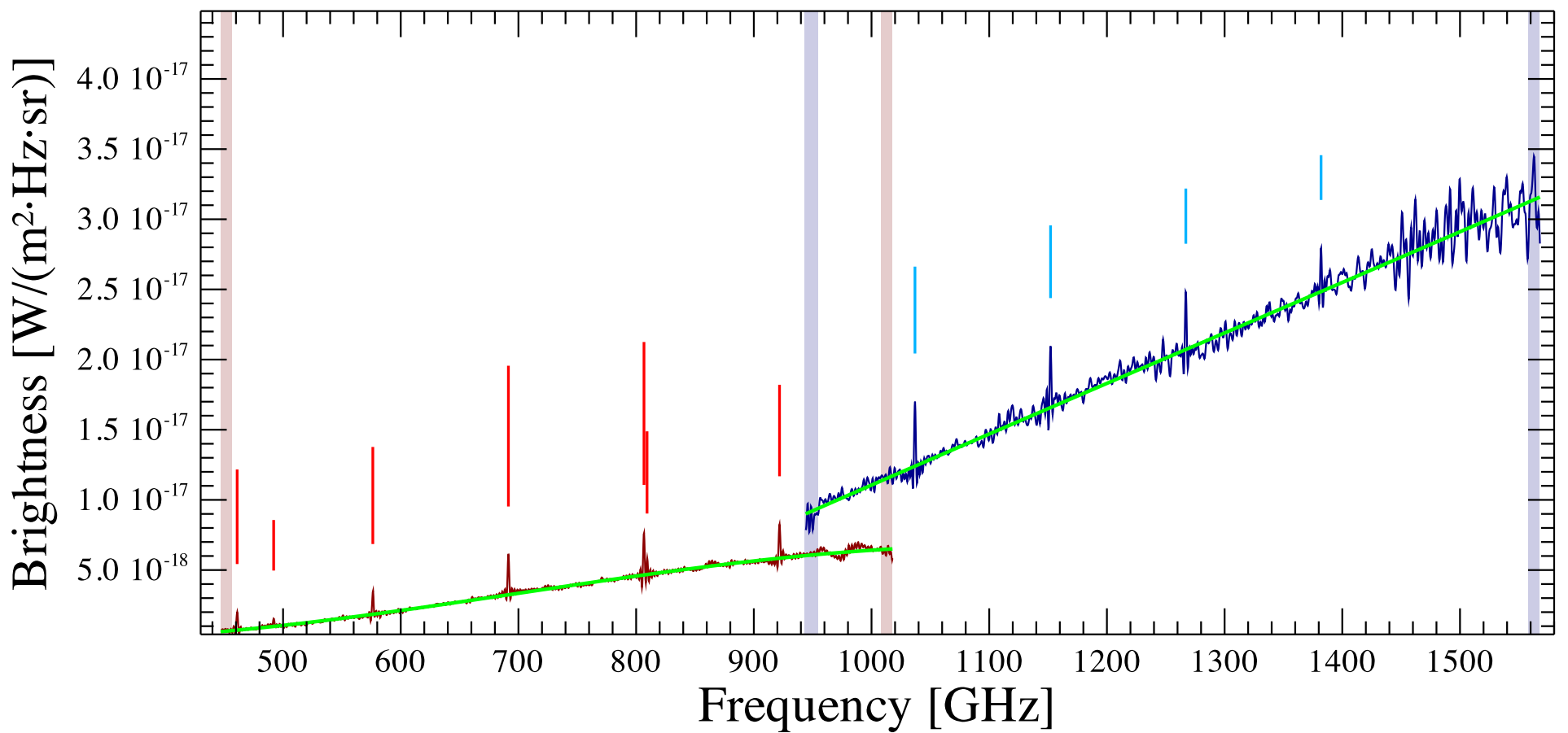
RNO 91 Observation ID 1342251285; (7/4)
