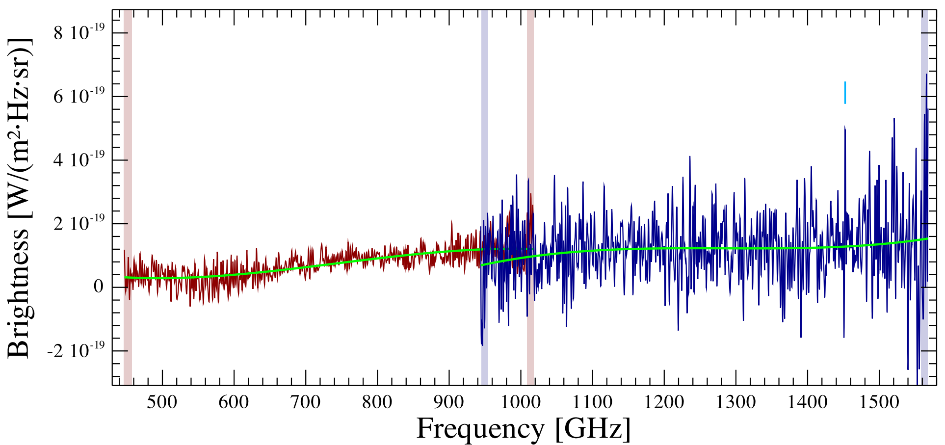
NGC1275-offset2 Observation ID 1342250529; (0/1)
