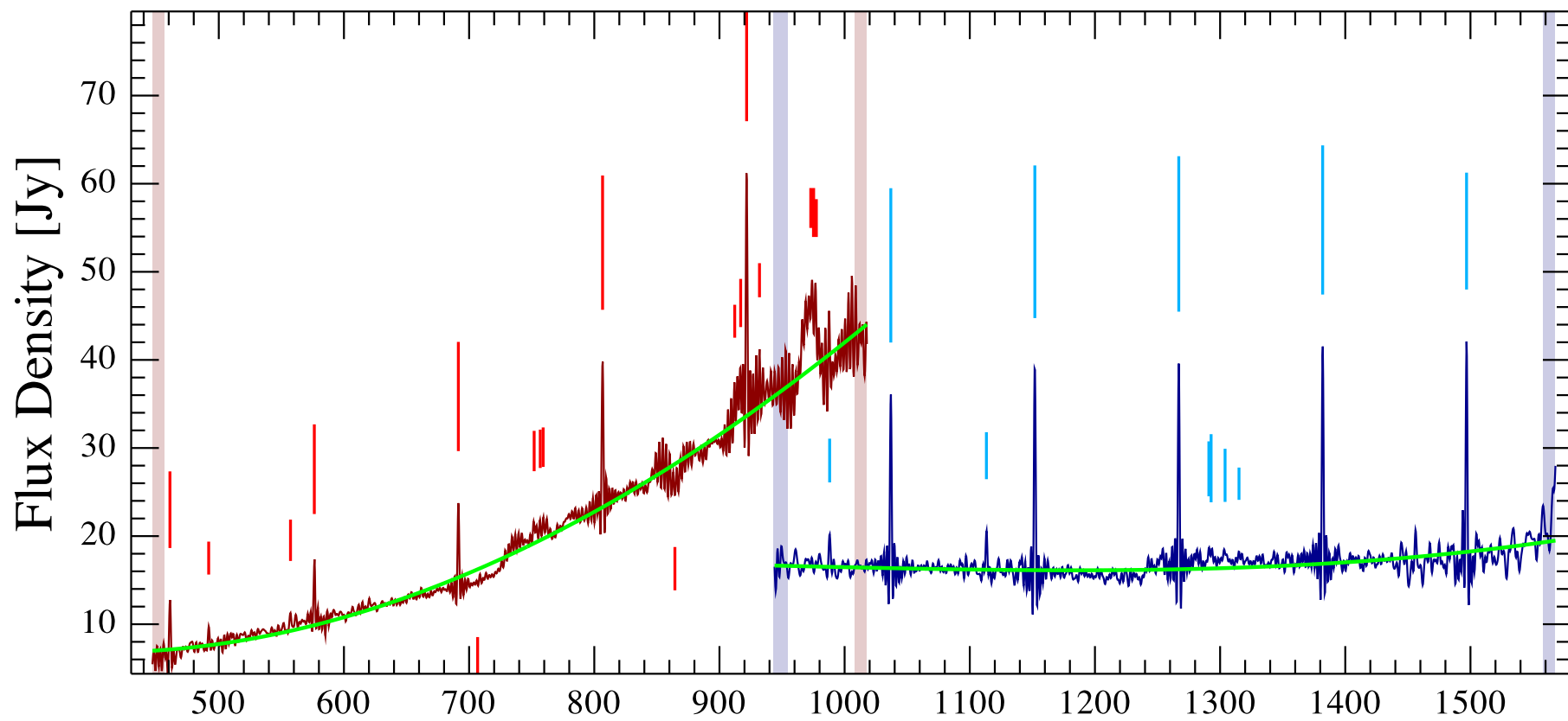
IRAS 15398/B228 Observation ID 1342250515; (8/8)
