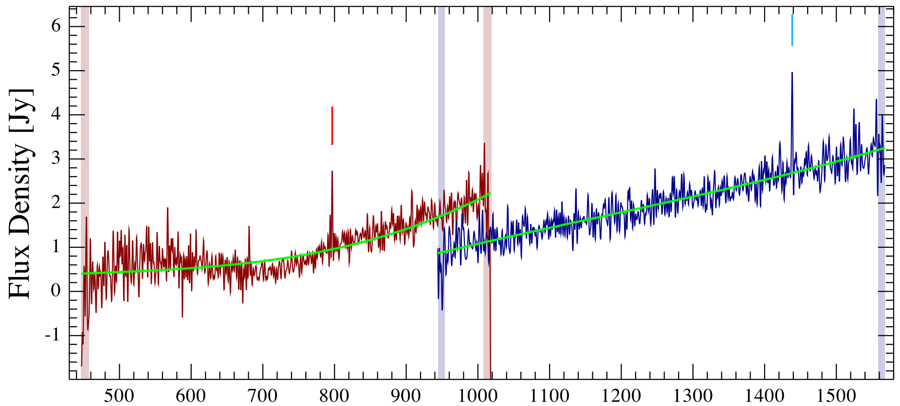
IC4518ABa Observation ID 1342250514; (1/1)
