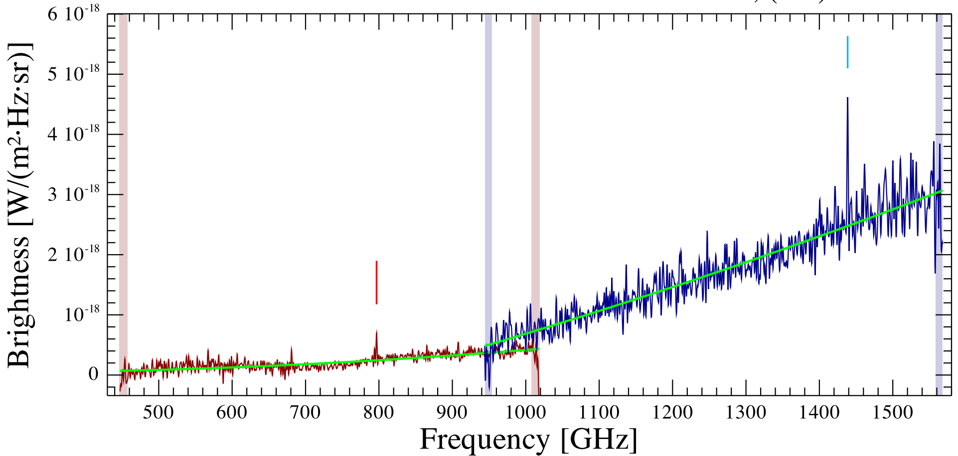
IC4518ABa Observation ID 1342250514; (1/1)
