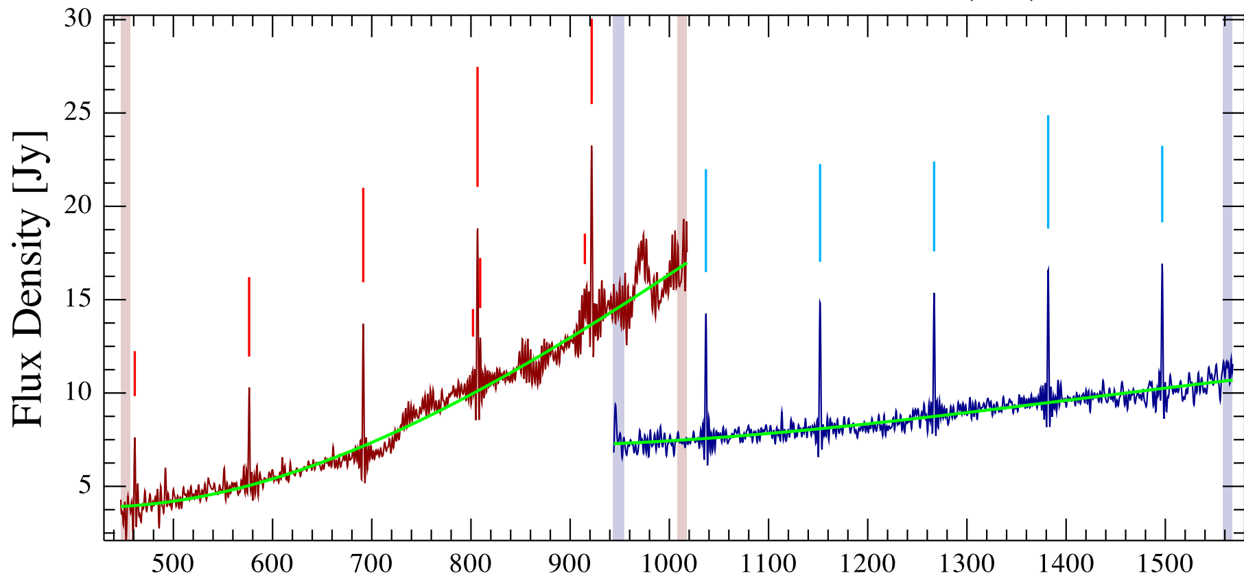
TMC 1 Observation ID 1342250512; (7/5)
