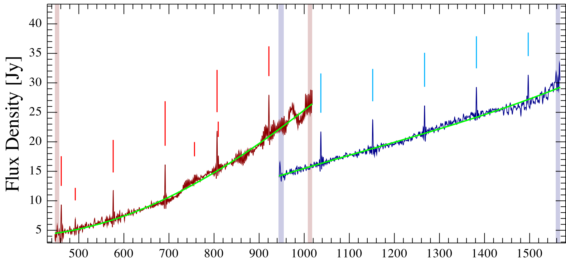
TMC 1A Observation ID 1342250510; (8/4)
