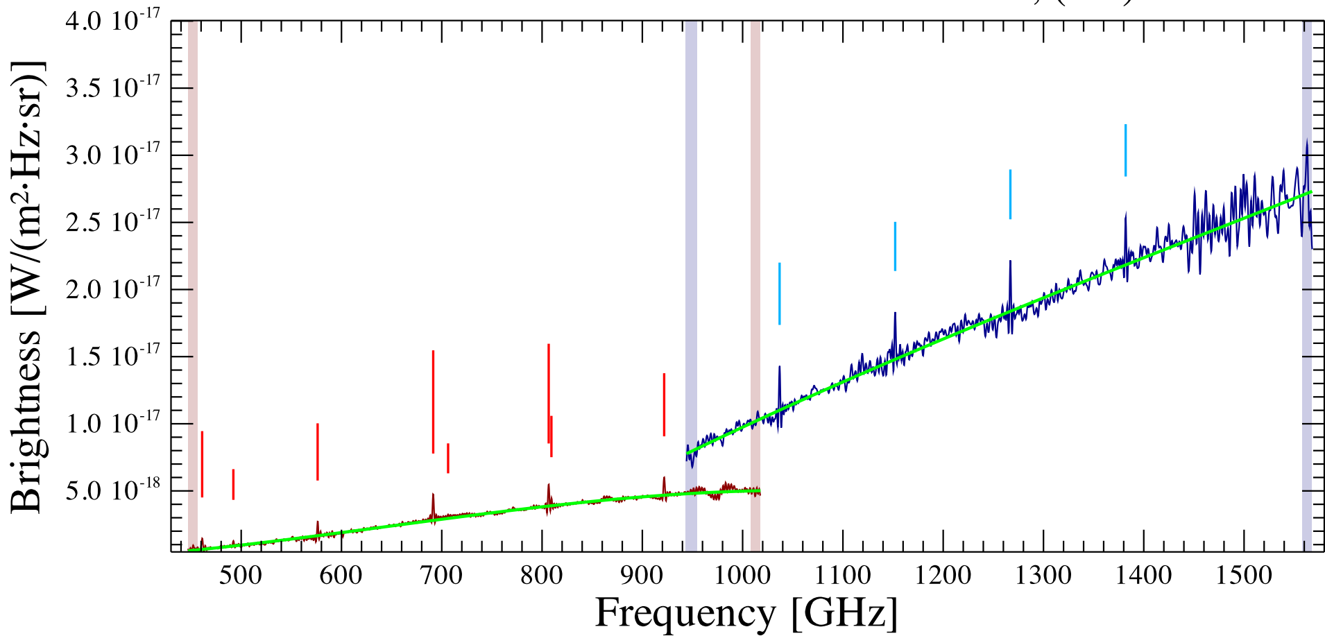
TMC 1A Observation ID 1342250510; (8/4)
