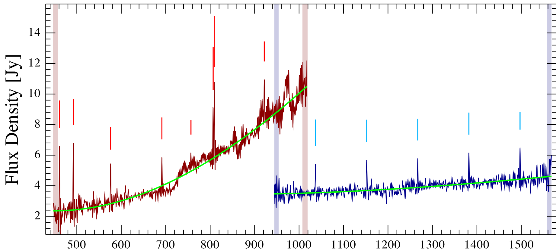
IRAS03301+3111 Observation ID 1342249477; (7/5)
