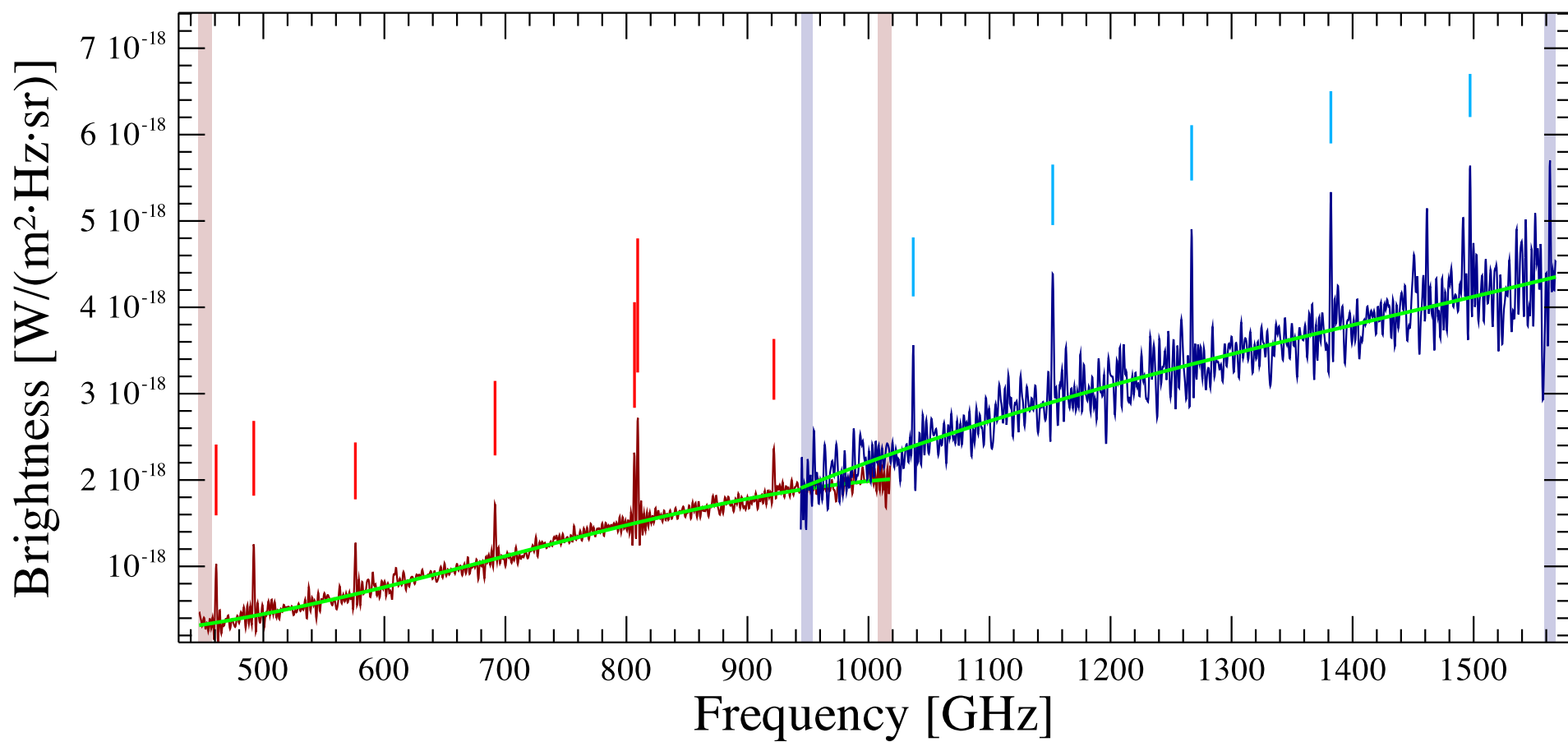
IRAS03301+3111 Observation ID 1342249477; (7/5)
