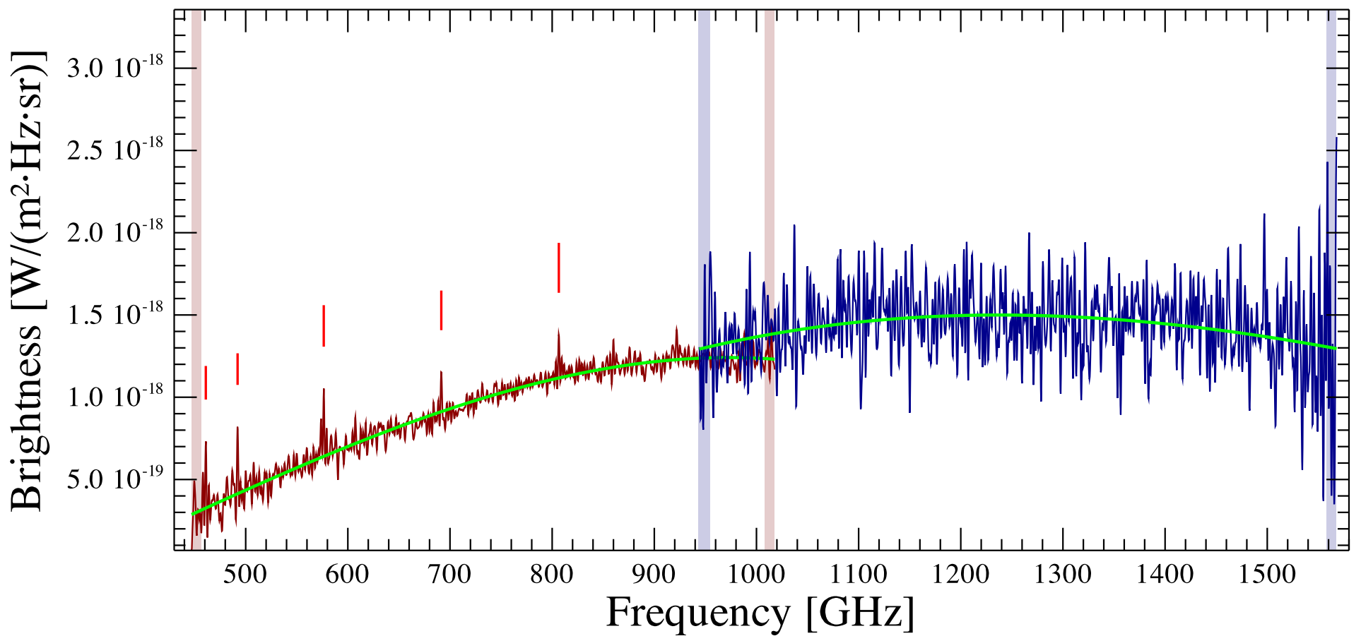
L1455-IRS3 Observation ID 1342249474; (5/0)
