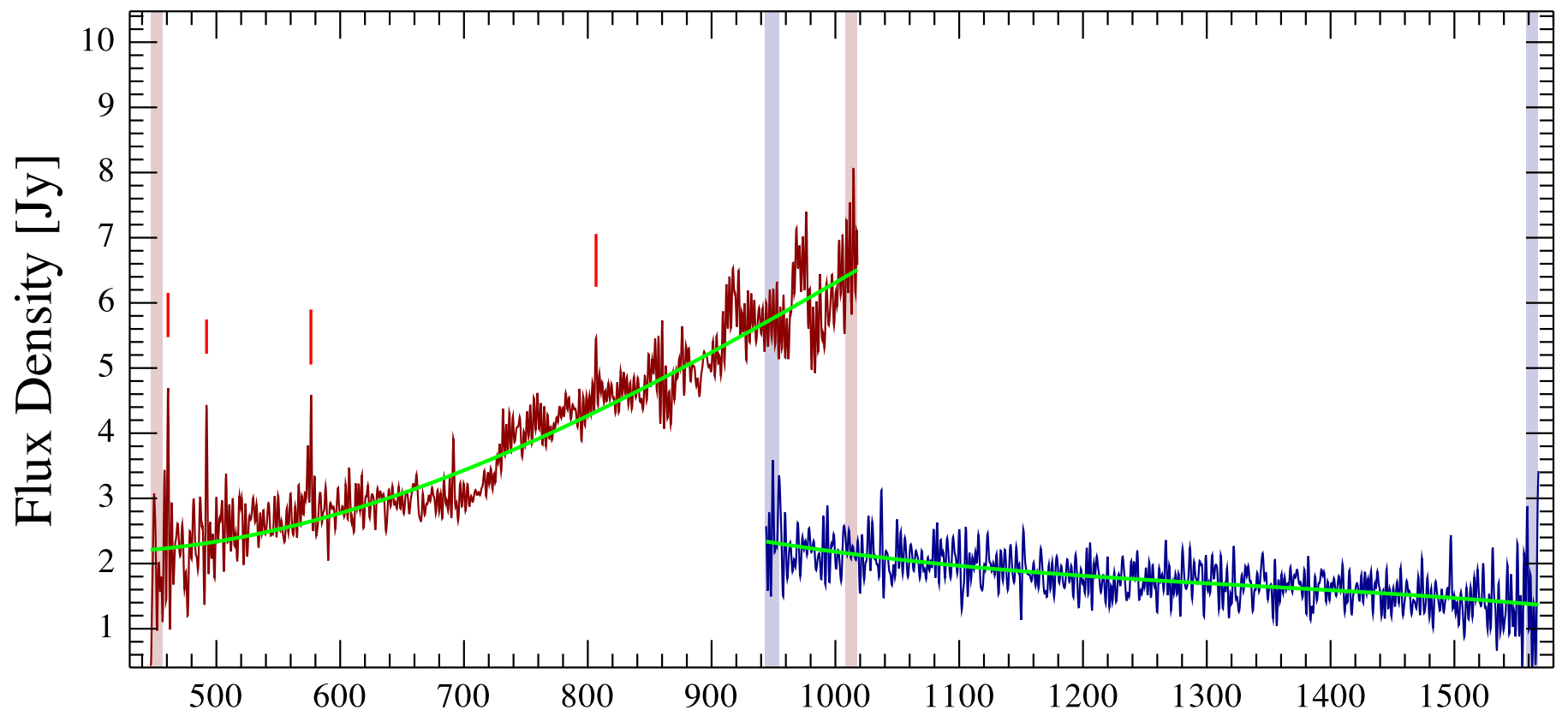
L1455-IRS3 Observation ID 1342249474; (5/0)
