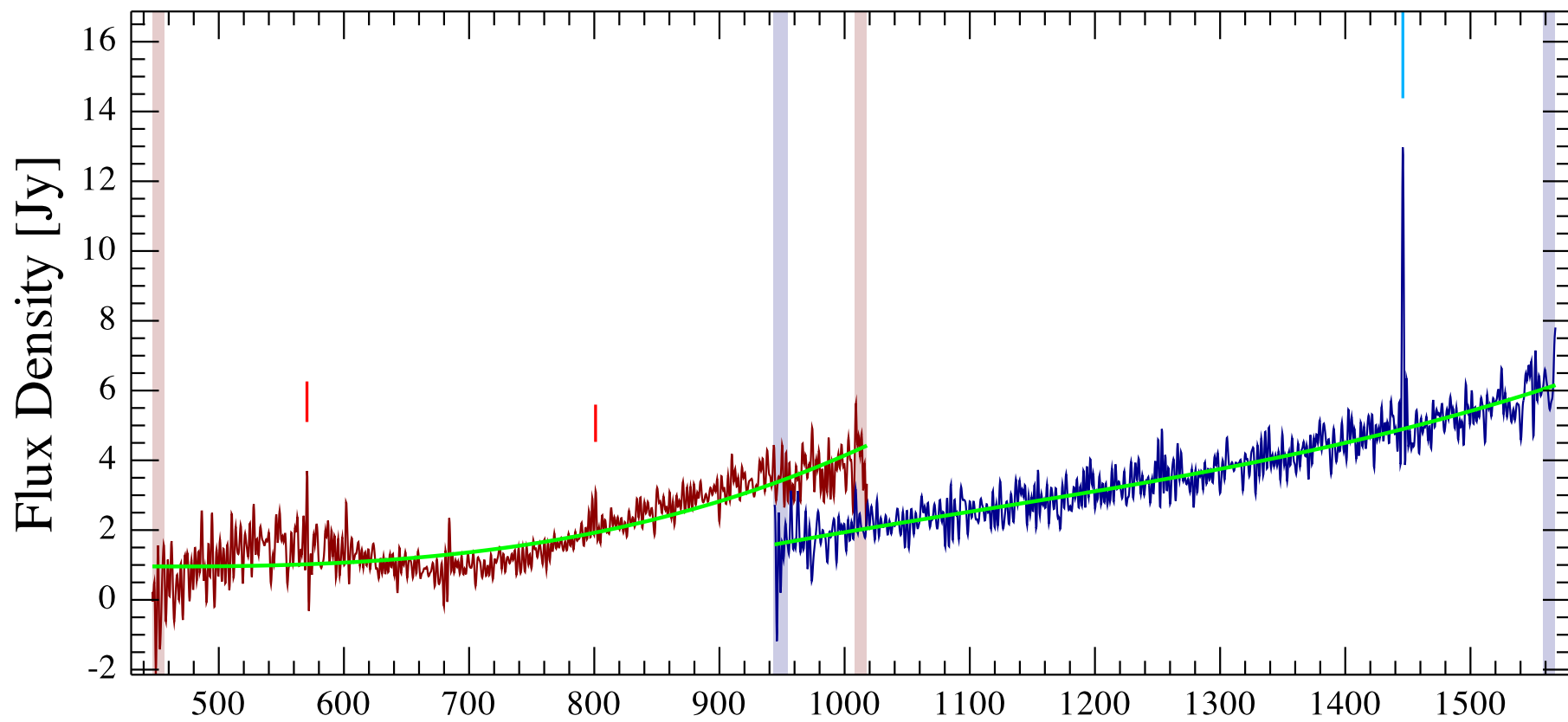
ESO221-IG010 Observation ID 1342249461; (4/1)
