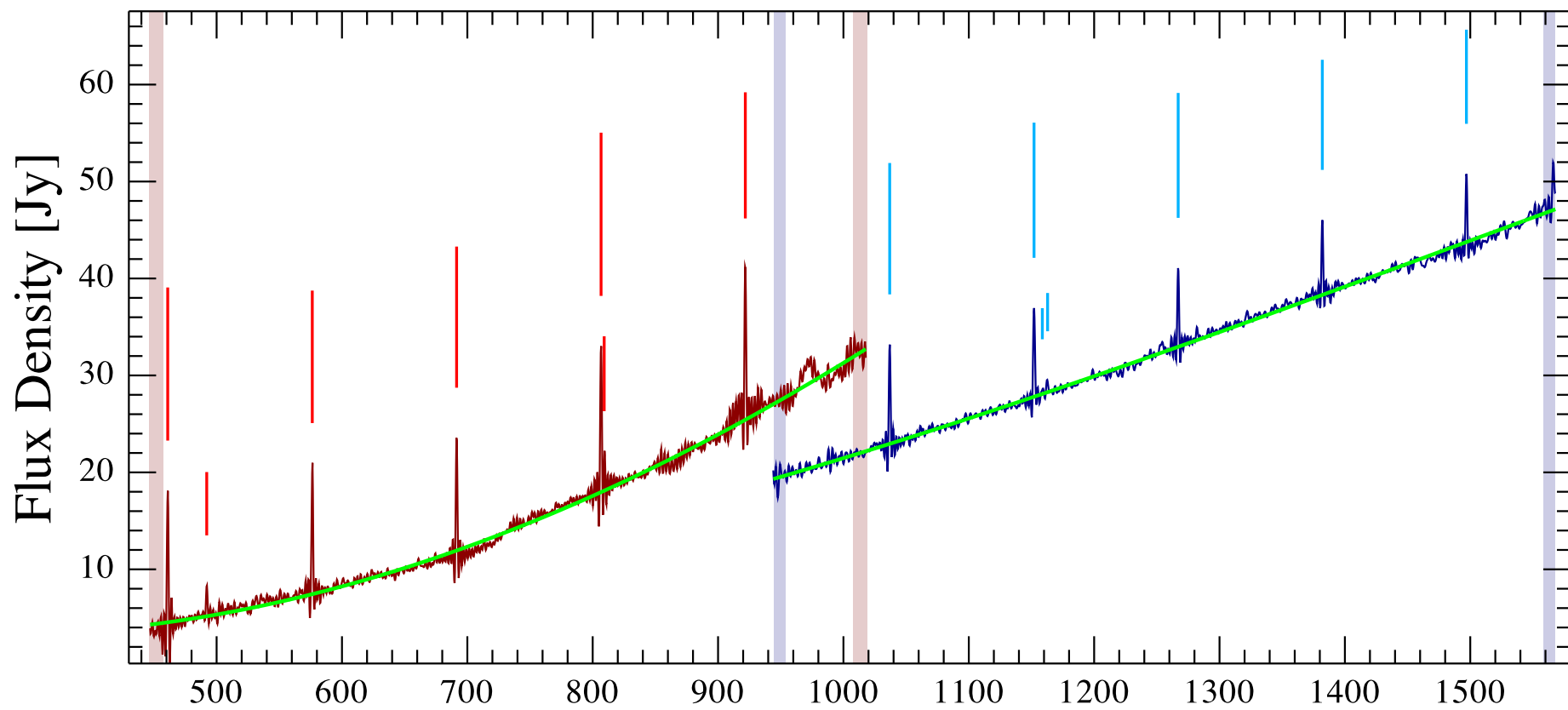
IRAS03245+3002 Observation ID 1342249053; (9/9)
