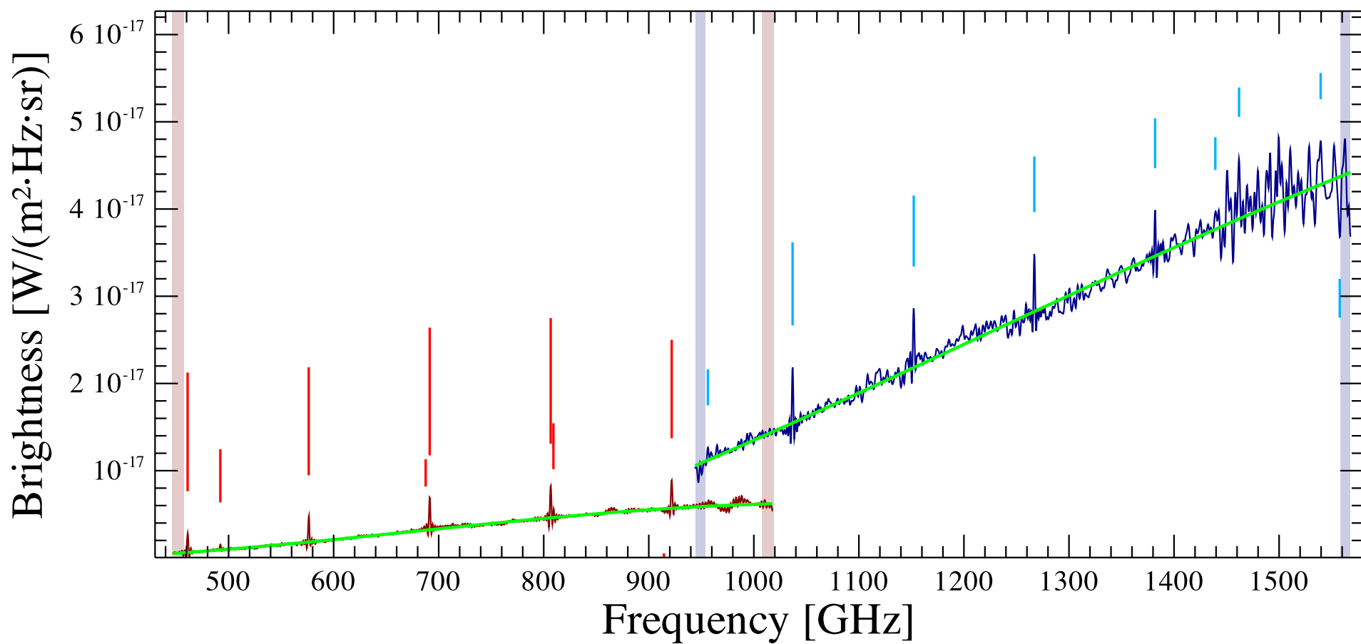
IRAS03245+3002 Observation ID 1342249053; (9/9)
