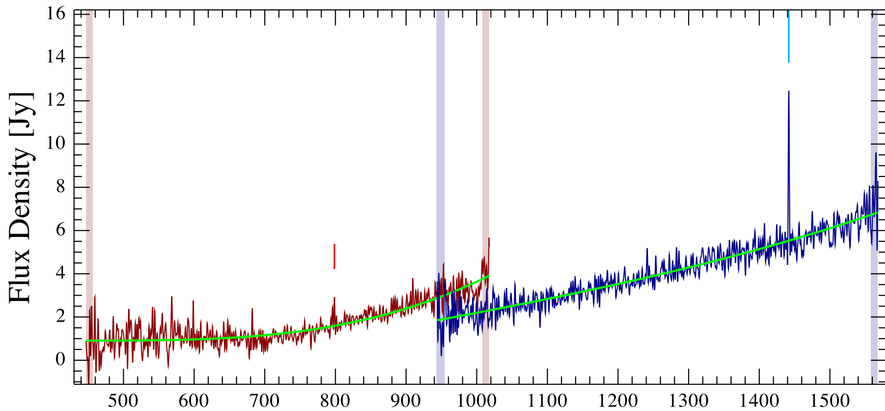
NGC5936 Observation ID 1342249046; (2/1)
