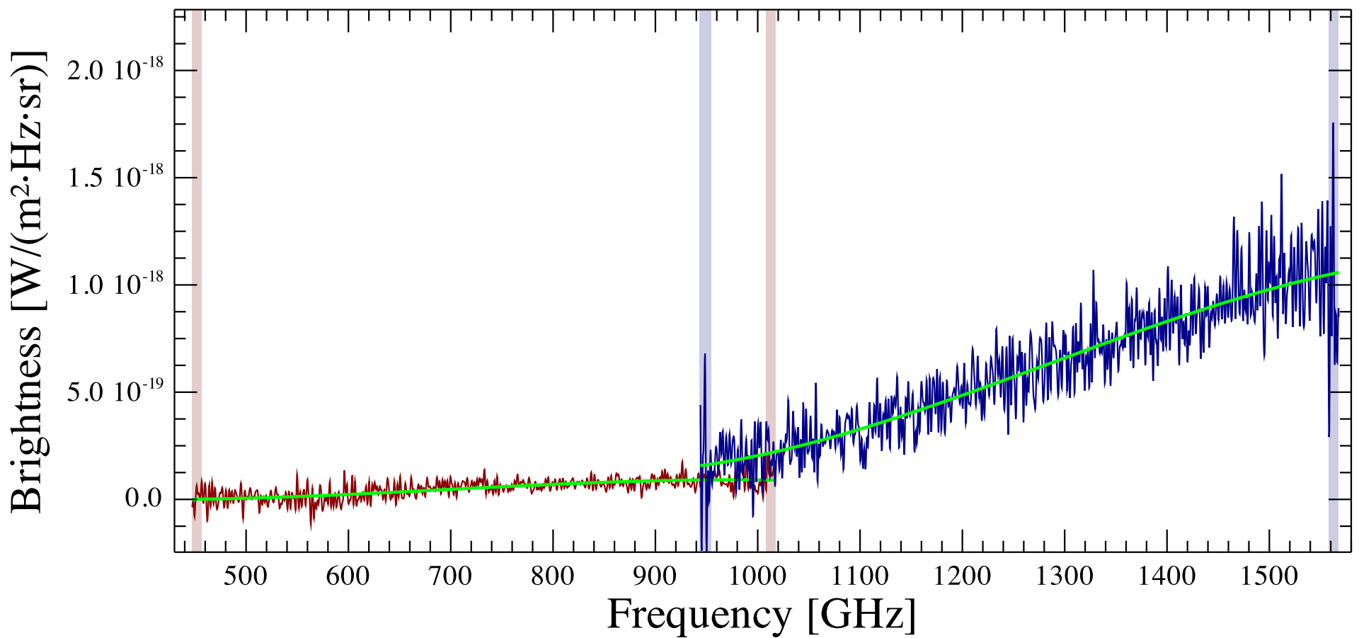
IRAS 15462-0450 Observation ID 1342249045; (0/0)
