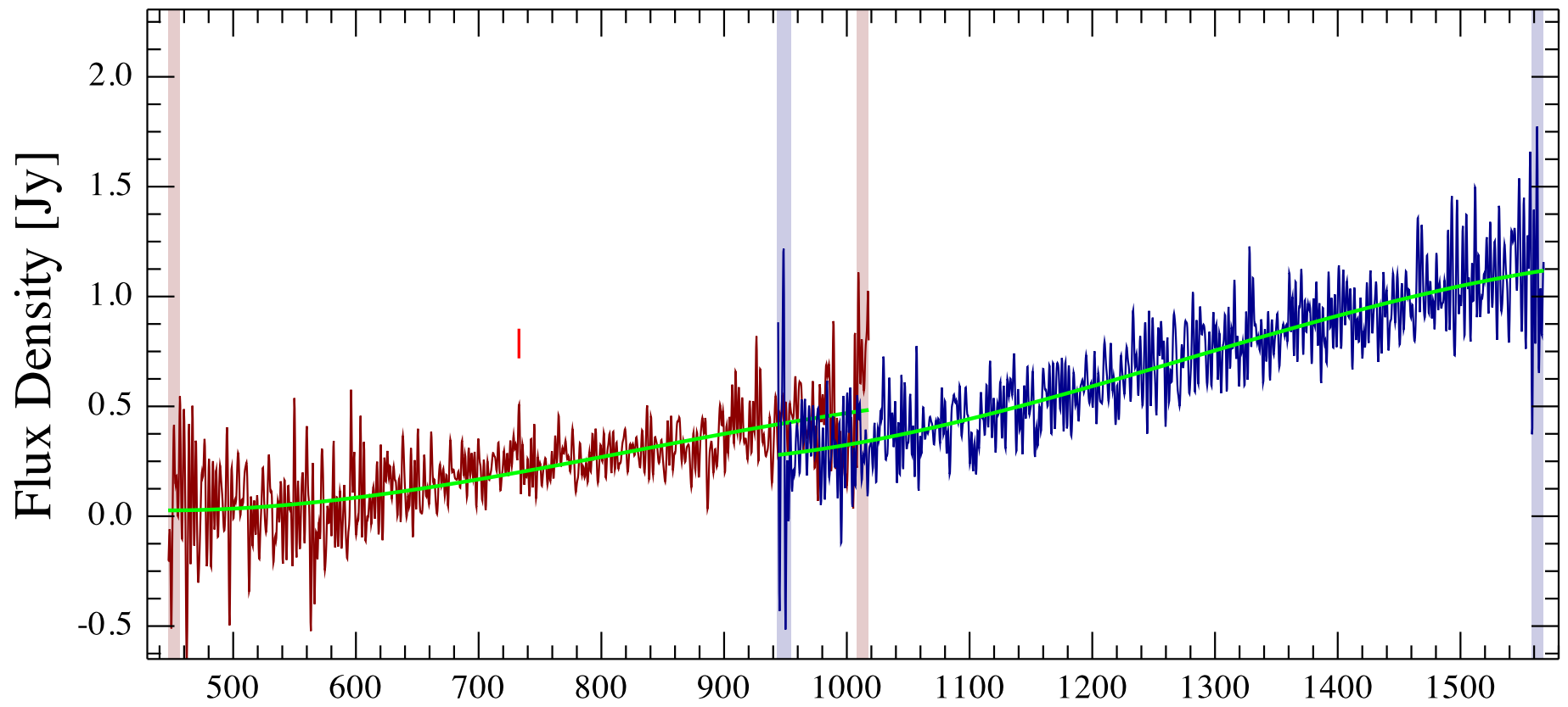
IRAS 15462-0450 Observation ID 1342249045; (0/0)
