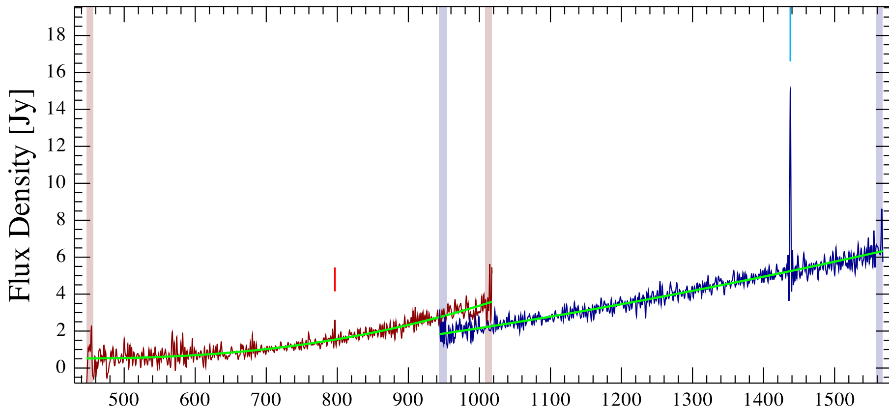
IC4280 Observation ID 1342249042; (1/1)
