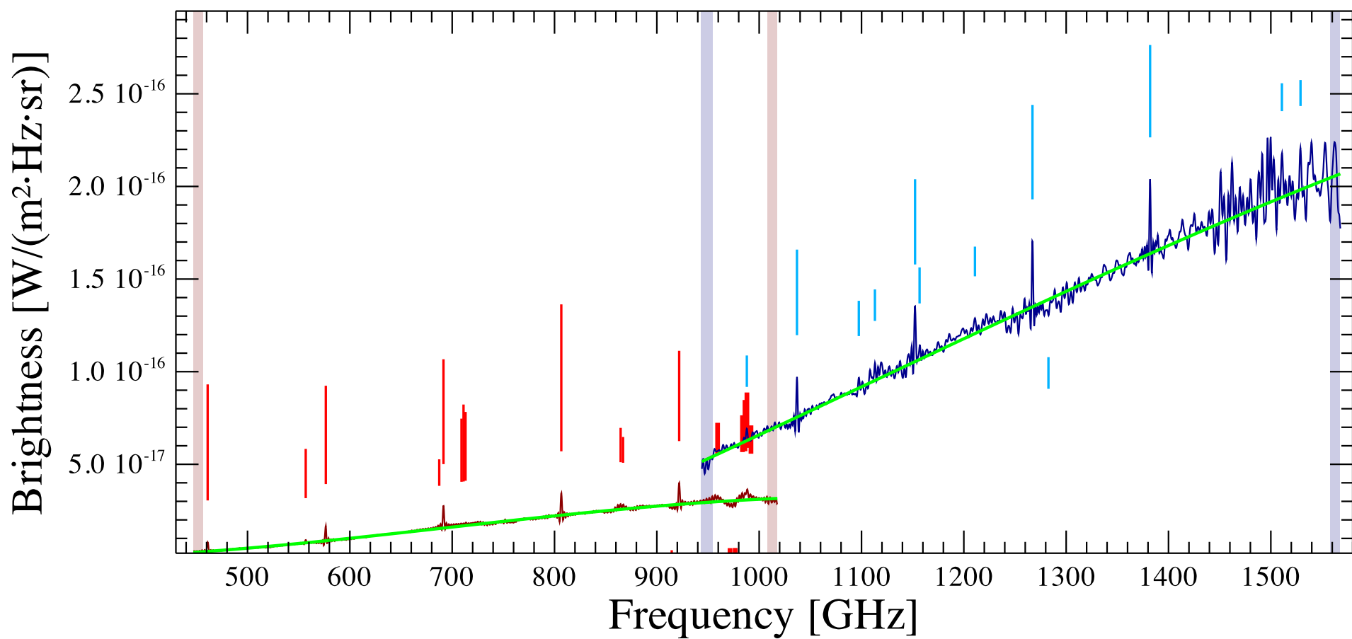
BHR 71 Observation ID 1342248249; (21/12)
